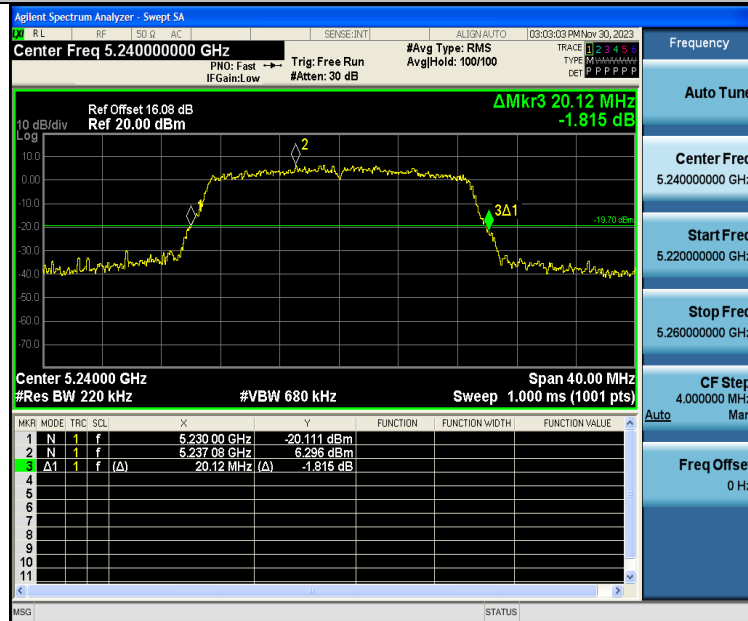
11AC20SISO-Ant1-5240
