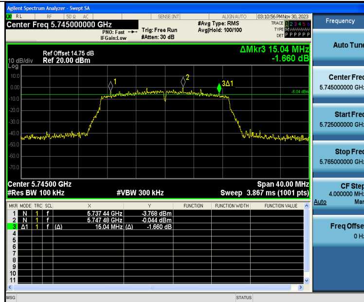
11AC20SISO-Ant1-5745-PASS
