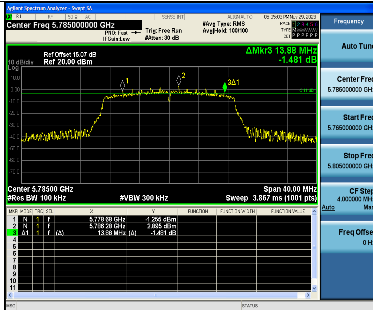
11N20SISO-Ant1-5785-PASS
