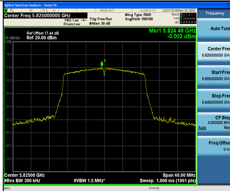
11N20SISO-Ant1-5825-PASS
