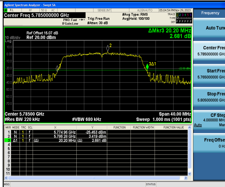
11N20SISO-Ant1-5785
