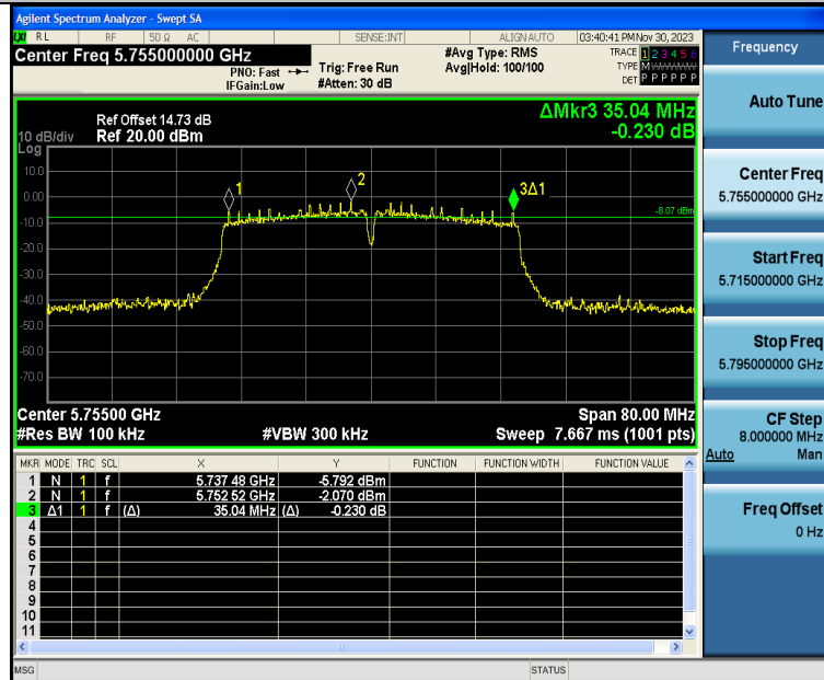
11AC40SISO-Ant1-5755-PASS
