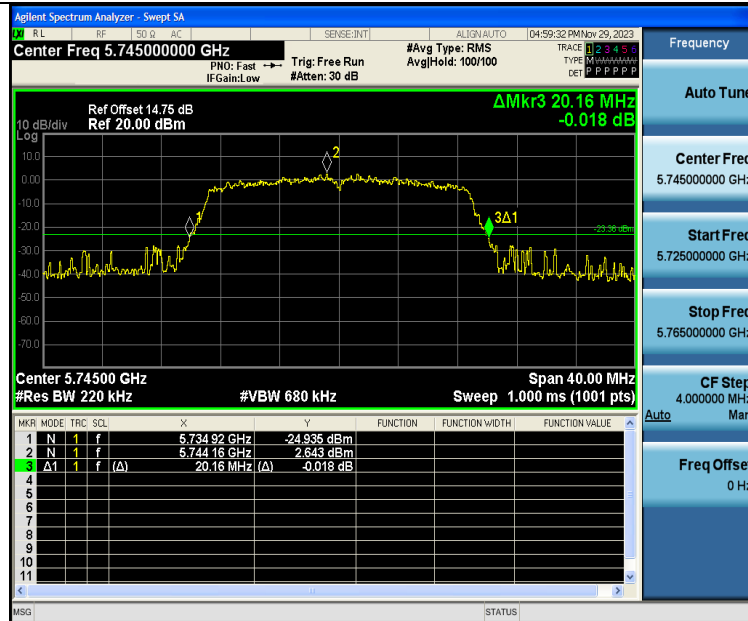
11N20SISO-Ant1-5745
