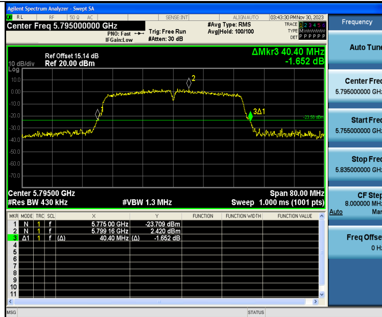
11AC40SISO-Ant1-5795
