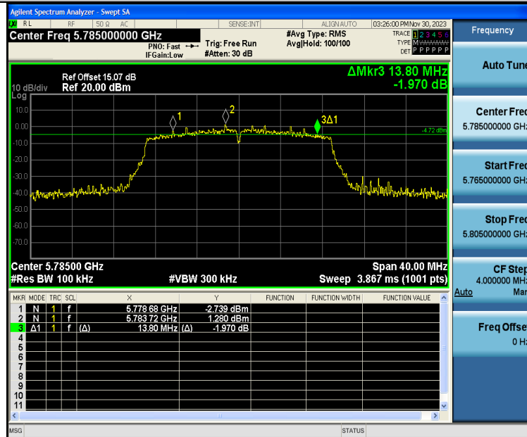
11AC20SISO-Ant1-5785-PASS
