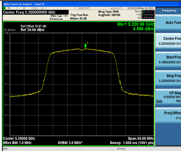
11AC20SISO-Ant1-5200-PASS
