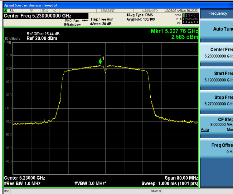
11N40SISO-Ant1-5230-PASS
