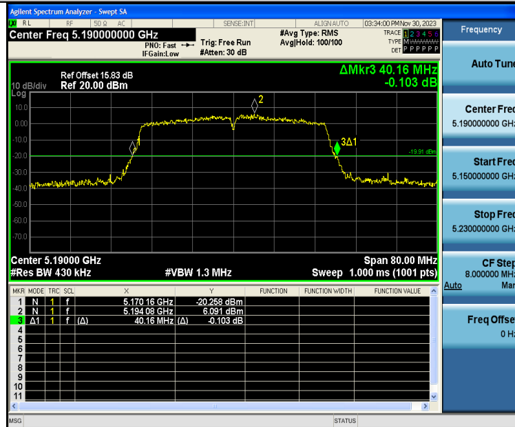
11AC40SISO-Ant1-5190
