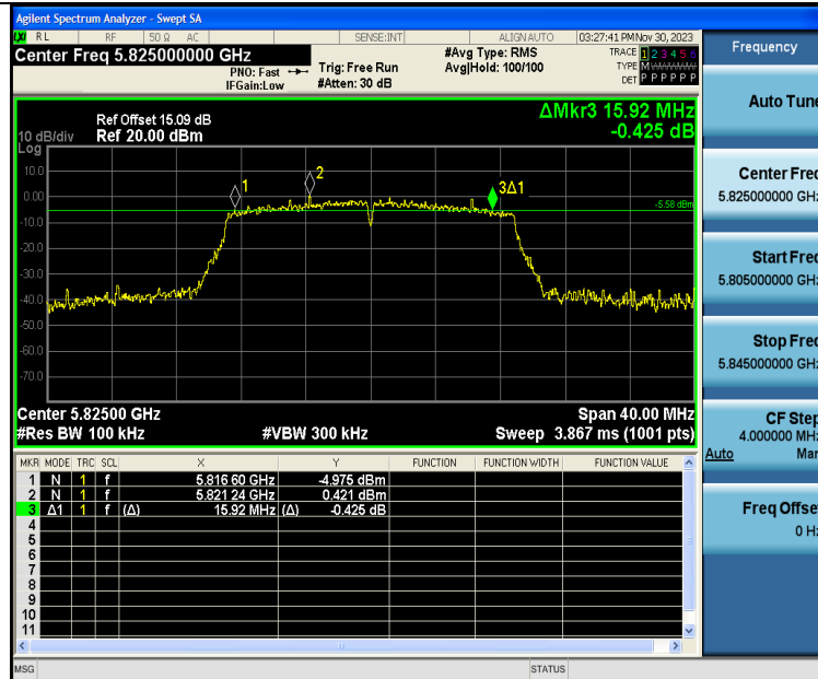
11AC20SISO-Ant1-5825-PASS
