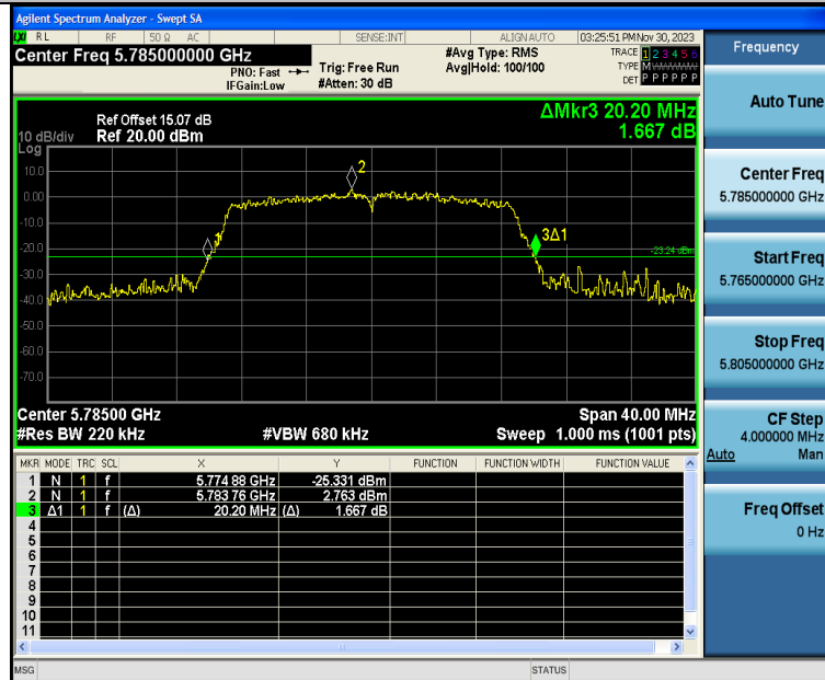
11AC20SISO-Ant1-5785
