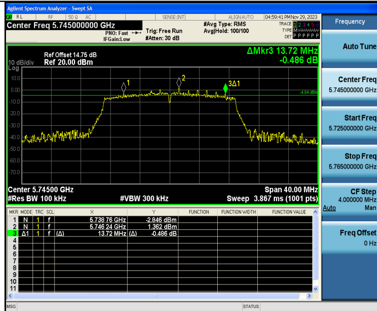
11N20SISO-Ant1-5745-PASS
