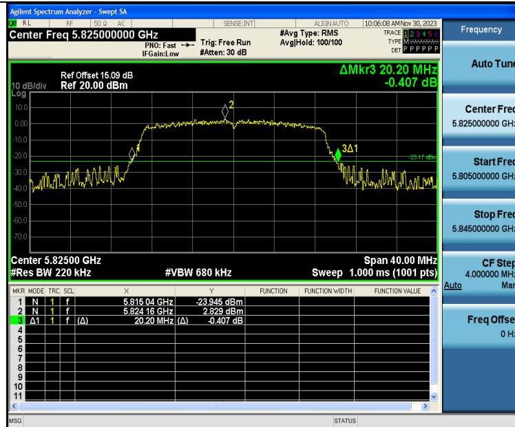
11N20SISO-Ant1-5825
