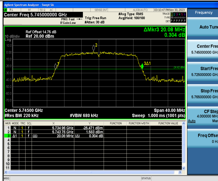
11AC20SISO-Ant1-5745
