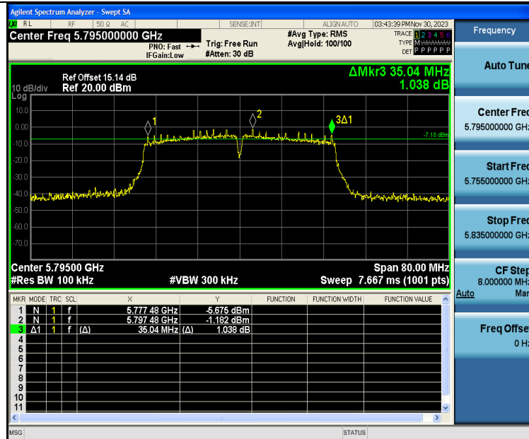
11AC40SISO-Ant1-5795-PASS
