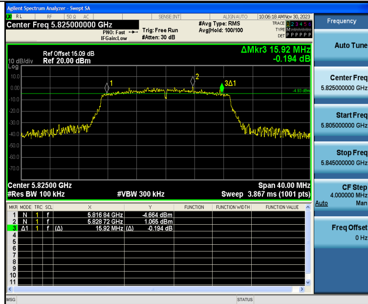
11N20SISO-Ant1-5825-PASS
