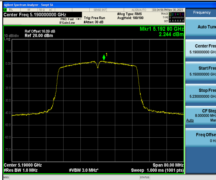
11AC40SISO-Ant1-5190-PASS
