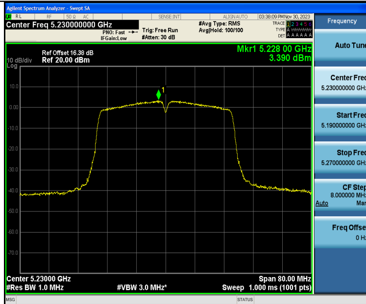
11AC40SISO-Ant1-5230-PASS
