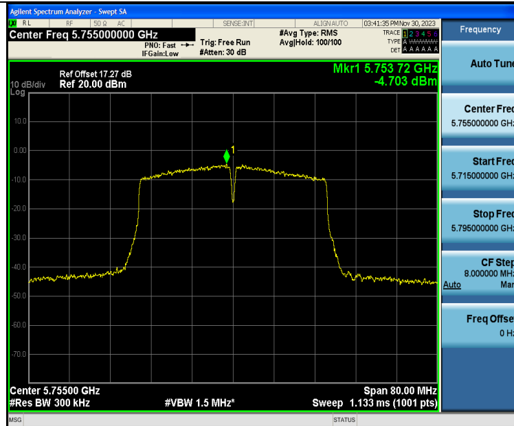
11AC40SISO-Ant1-5755-PASS
