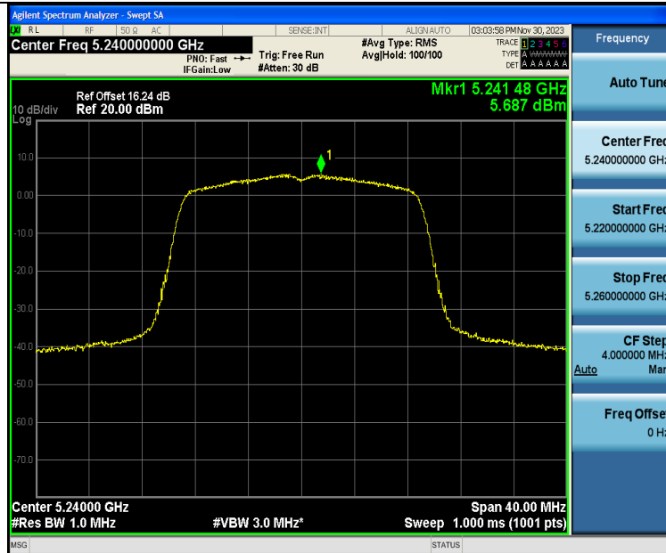
11AC20SISO-Ant1-5240-PASS
