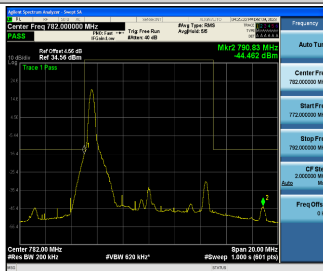
Band13-10MHz-QPSK-23230-1RB#49
