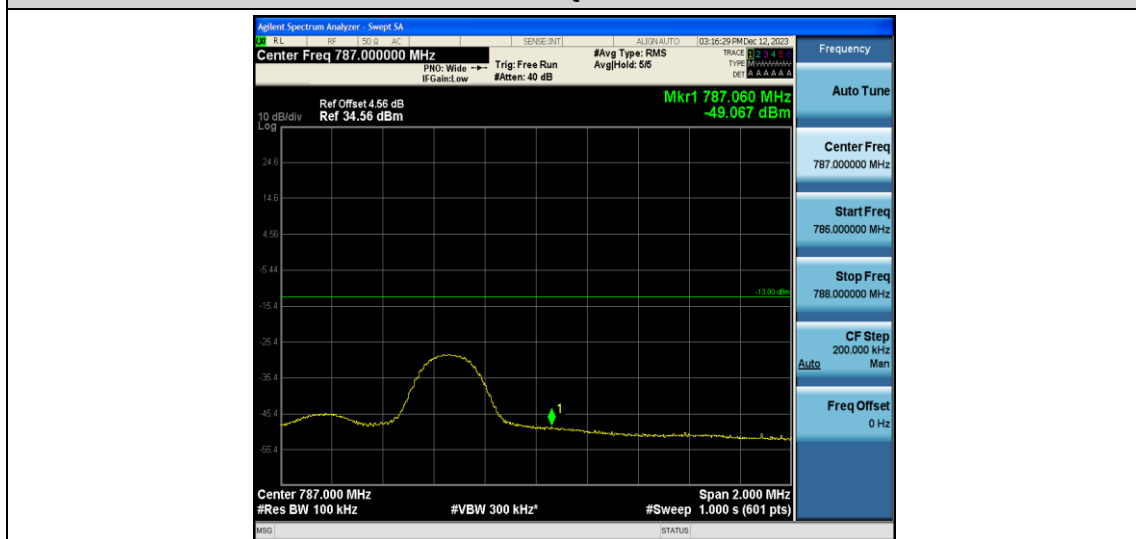
Band13-5MHz-16QAM-23255-1RB#24
