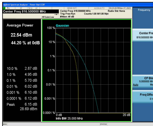
Band26-5MHz-16QAM-26715-25RB#0
