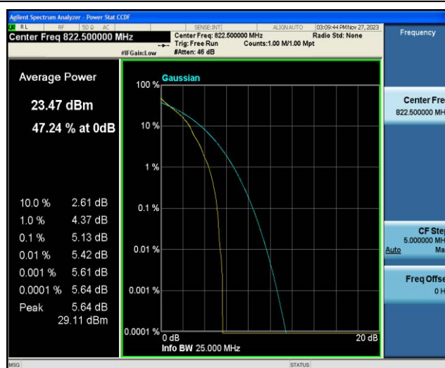
Band26-3MHz-QPSK-26775-15RB#0
