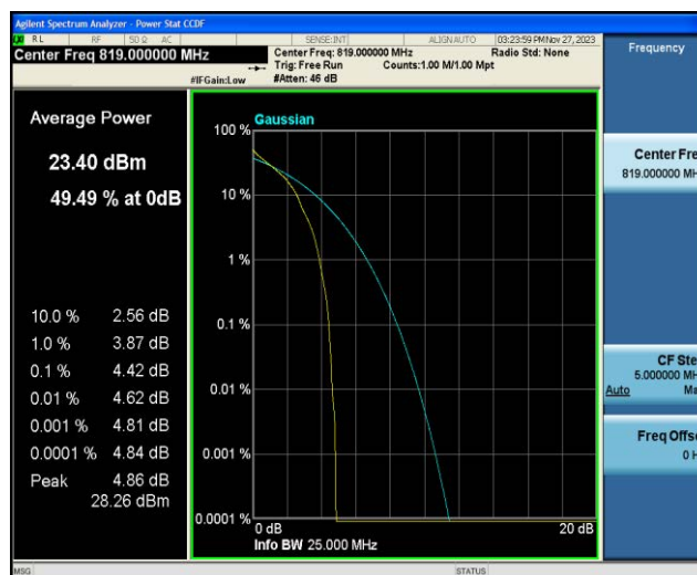
Band26-5MHz-QPSK-26740-25RB#0
