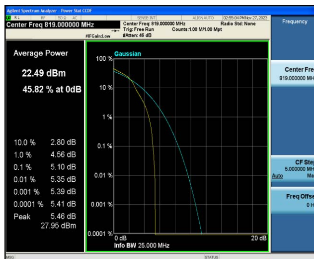
Band26-1.4MHz-16QAM-26740-6RB#0
