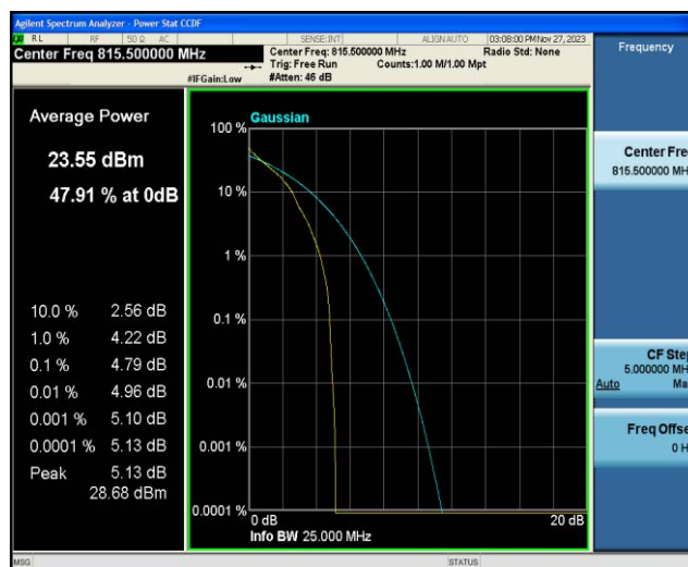
Band26-3MHz-QPSK-26705-15RB#0
