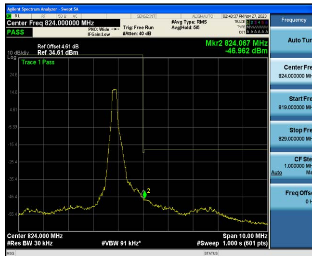
Band26-1.4MHz-QPSK-26783-1RB#5
