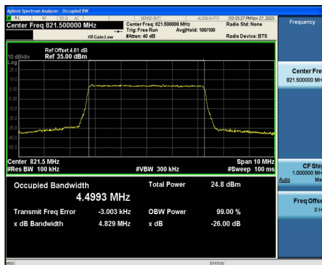
Band26-5MHz-16QAM-26715-25RB#0
