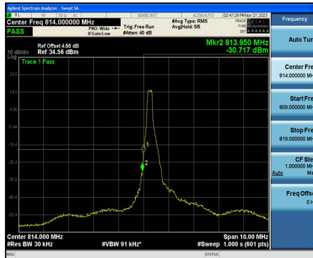
Band26-1.4MHz-16QAM-26697-1RB#5
