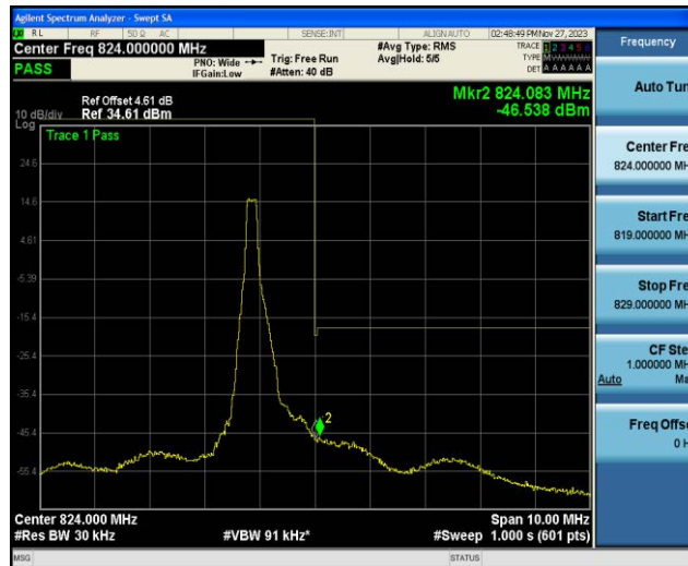
Band26-1.4MHz-16QAM-26783-1RB#5
