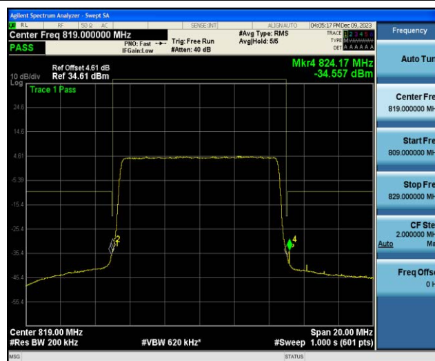
Band26-10MHz-16QAM-26740-1RB#0
