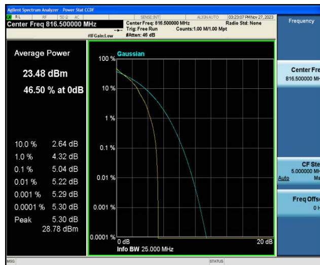
Band26-5MHz-QPSK-26715-25RB#0
