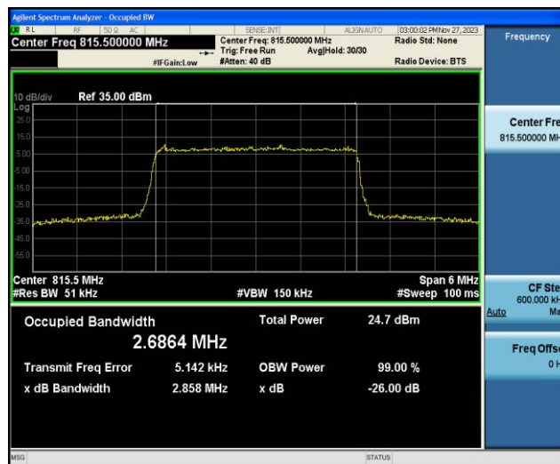
Band26-3MHz-QPSK-26740-15RB#0
