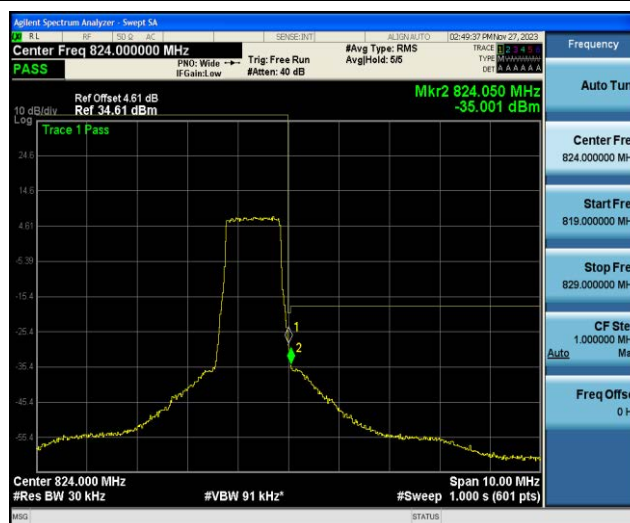
Band26-3MHz-QPSK-26705-1RB#0
