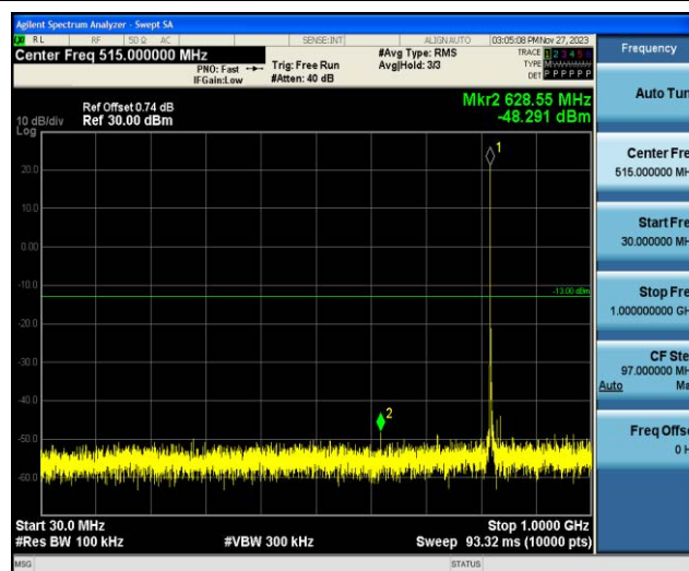
Band26-3MHz-QPSK-26775-1RB#0-Range2:1000~10000MHz
