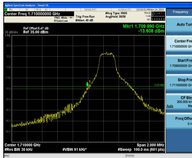
Band4-1.4MHz-QPSK-19957-1RB#5
