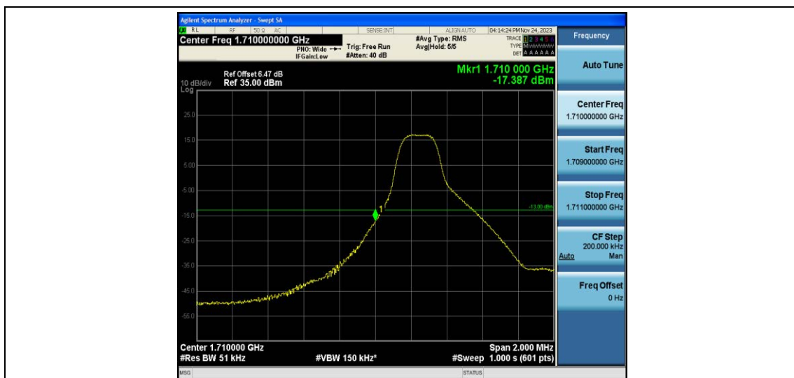
Band4-3MHz-16QAM-19965-1RB#14
