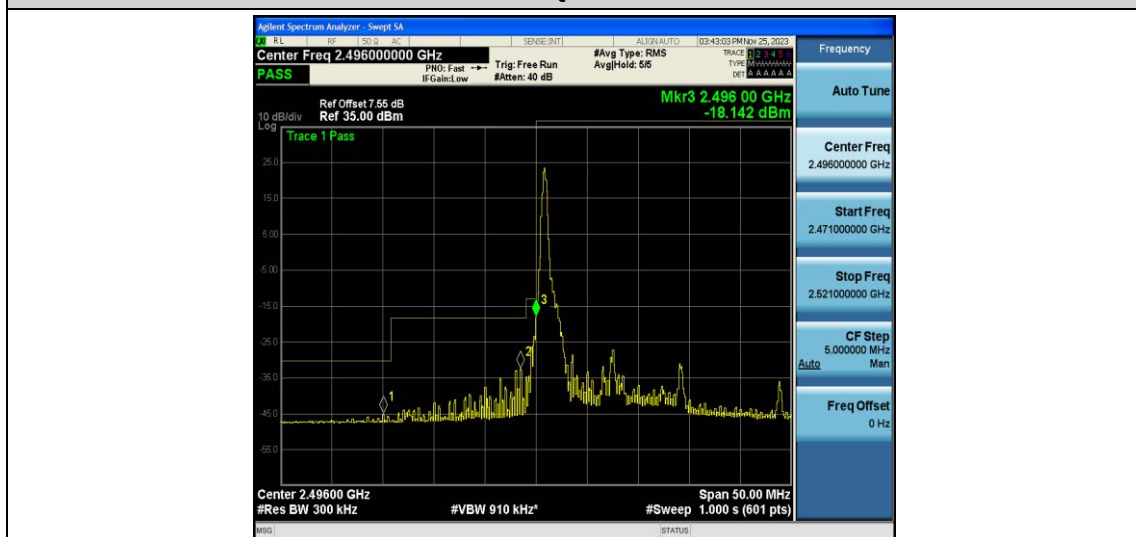
Band41-15MHz-QPSK-39725-1RB#74
