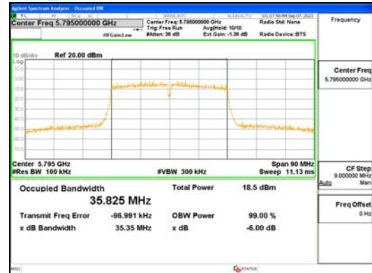
ANT 1_802.11ac_VHT40_UNII-3
