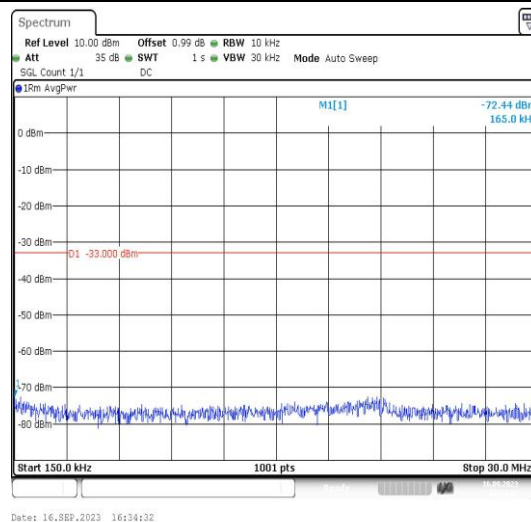
Band2-9262-4-0.15~30MHz-PASS
