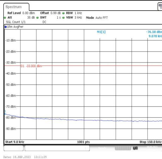
Band5-4182-4-0.009~0.15MHz-PASS
