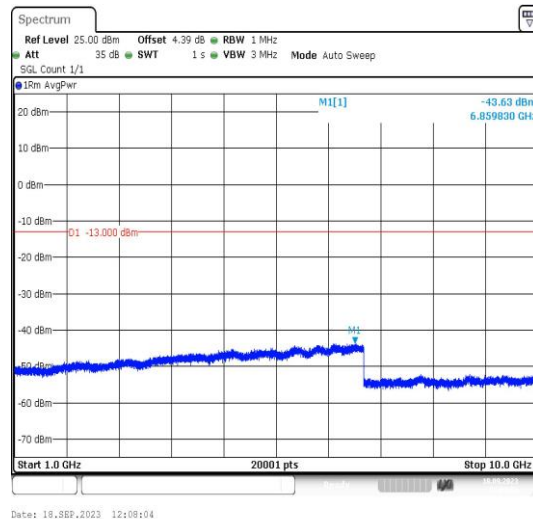
Band5-4132-3-1000~10000MHz-PASS
