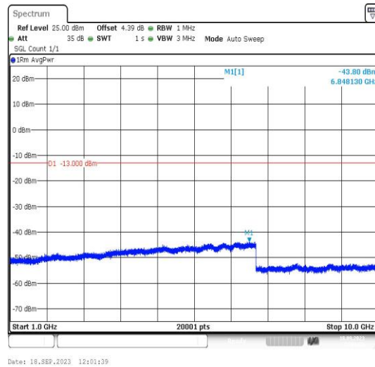
Band5-4132-1-1000~10000MHz-PASS
