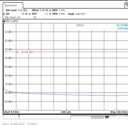
Band5-4182-3-0.009~0.15MHz-PASS
