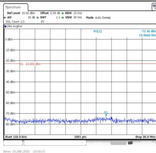
Band5-4182-1-0.15~30MHz-PASS
