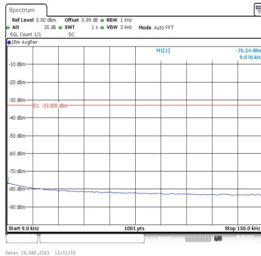
Band5-4182-1-0.009~0.15MHz-PASS
