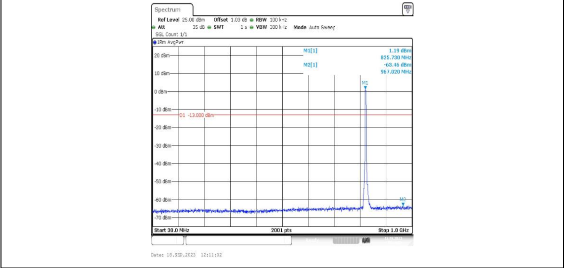
Band5-4132-4-30~1000MHz-PASS
