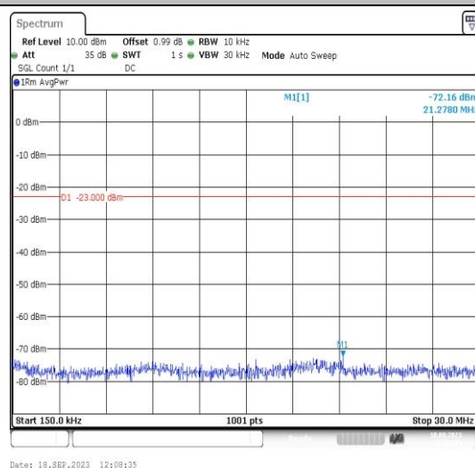
Band5-4182-3-0.15~30MHz-PASS
