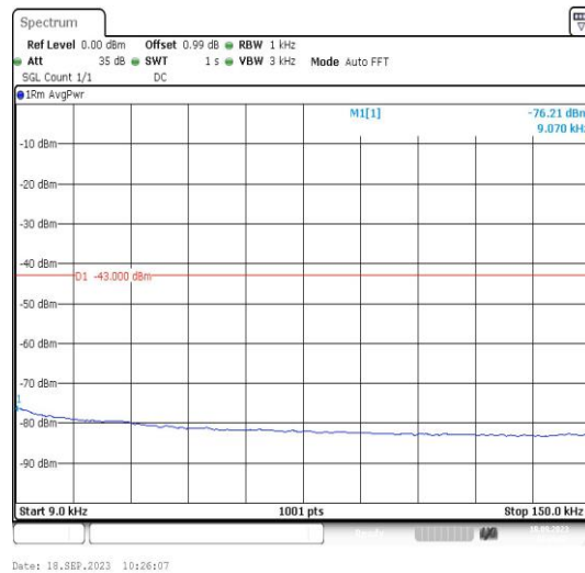
Band2-9400-4-0.009~0.15MHz-PASS
