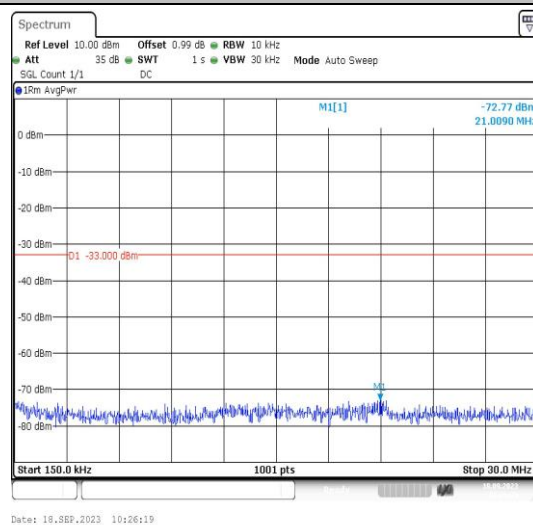
Band2-9400-4-0.15~30MHz-PASS
