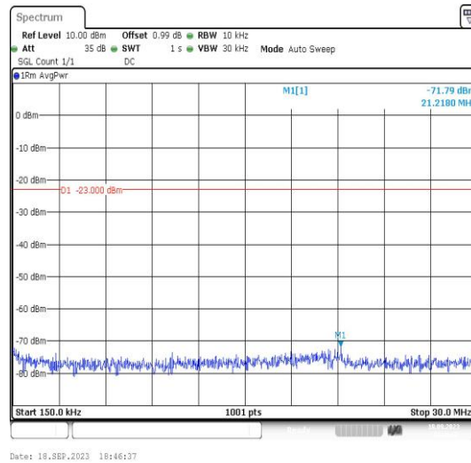
Band5-4233-2-0.15~30MHz-PASS
