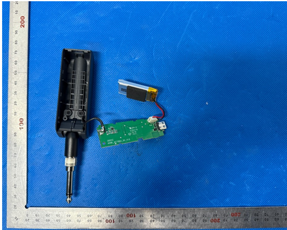
Open view-2 of EUT
