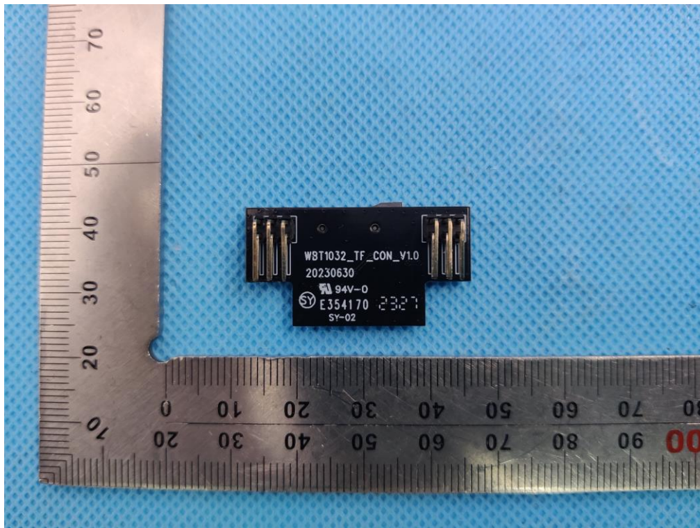
INTERNAL VIEW OF EUT (FIGURE 43)
