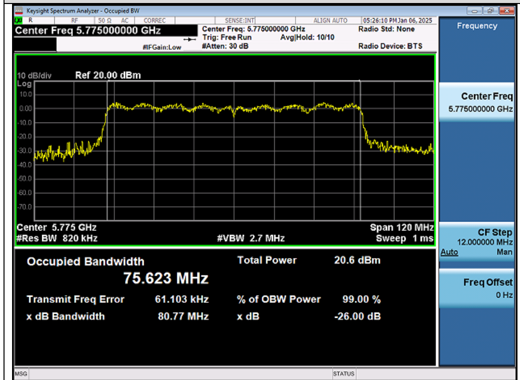
Test_Graph_802.11ac80_ANT1_5775_MCS0_OBW
