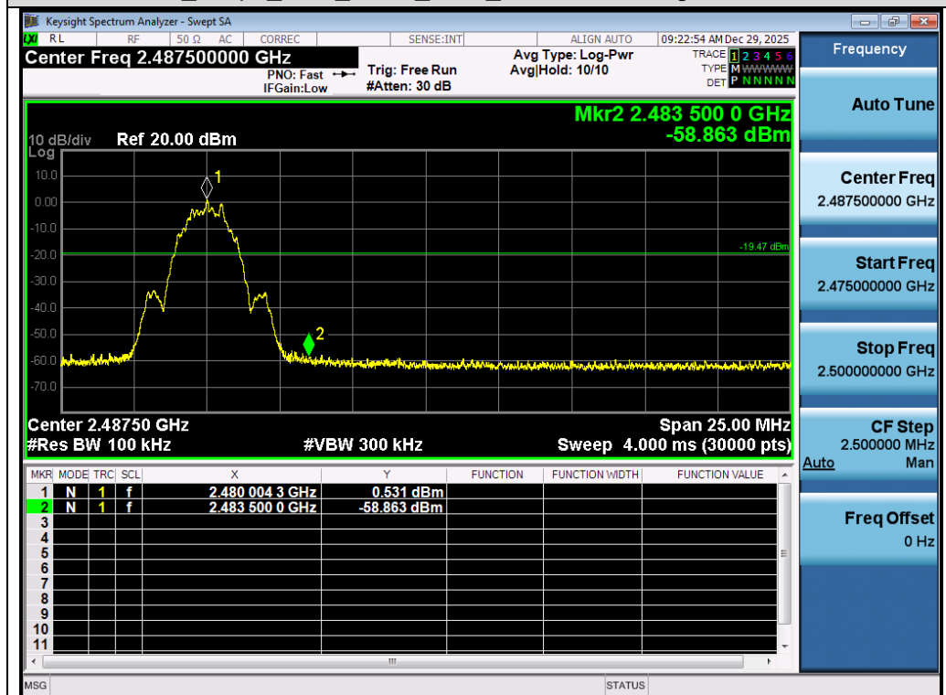
Test_Graph_SRD_ANT1_2480_Higher Band Edge Emissions
