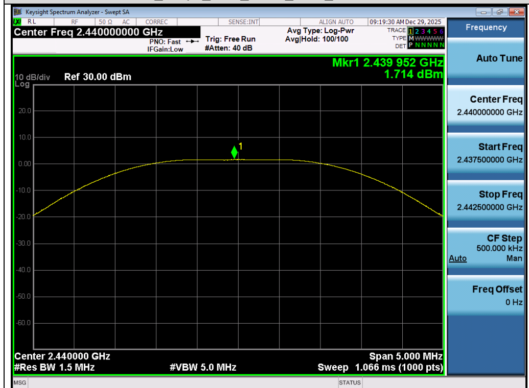
Test_Graph_SRD_ANT1_2440_Peak Power
