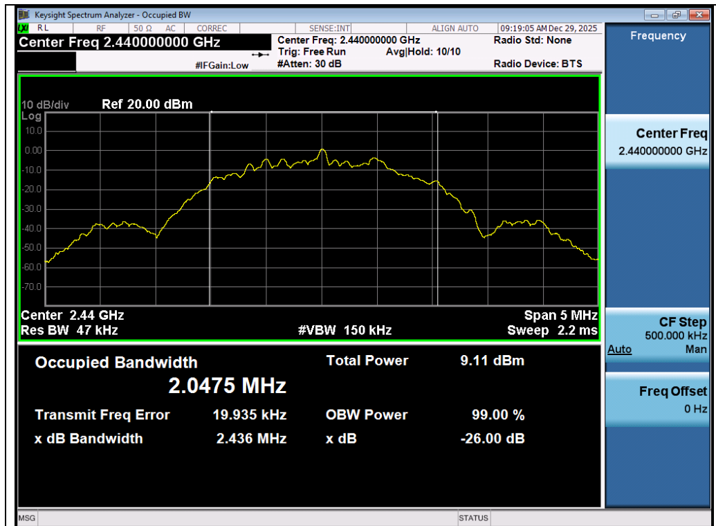
Test_Graph_SRD_ANT1_2440_OBW
