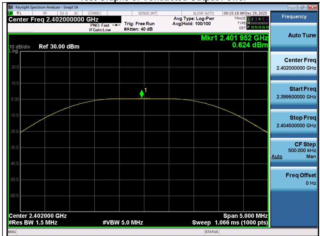
Test_Graph_SRD_ANT1_2402_Peak Power
