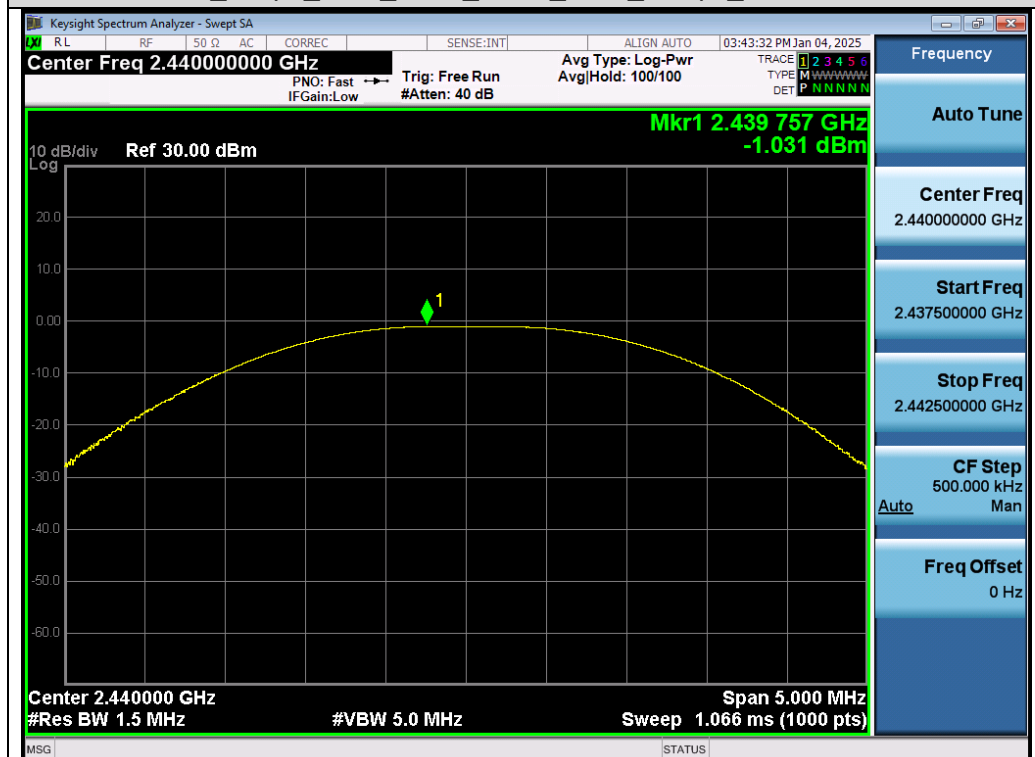
Test_Graph_2.4G_SRD_ANT1_2440_1Mbps_Peak Power
