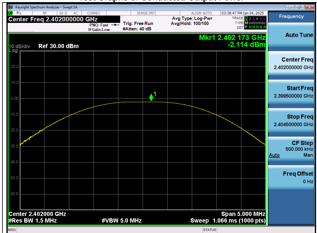
Test_Graph_2.4G_SRD_ANT1_2402_1Mbps_Peak Power
