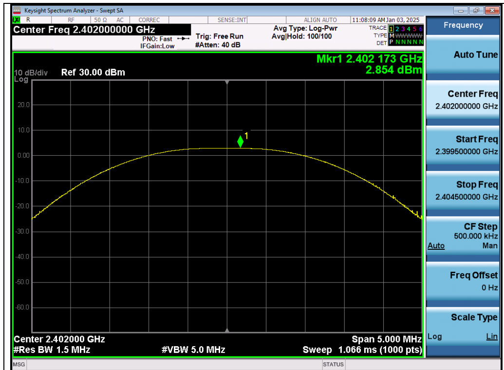
Test_Graph_2.4G_SRD_ANT4_2402_1Mbps_Peak Power
