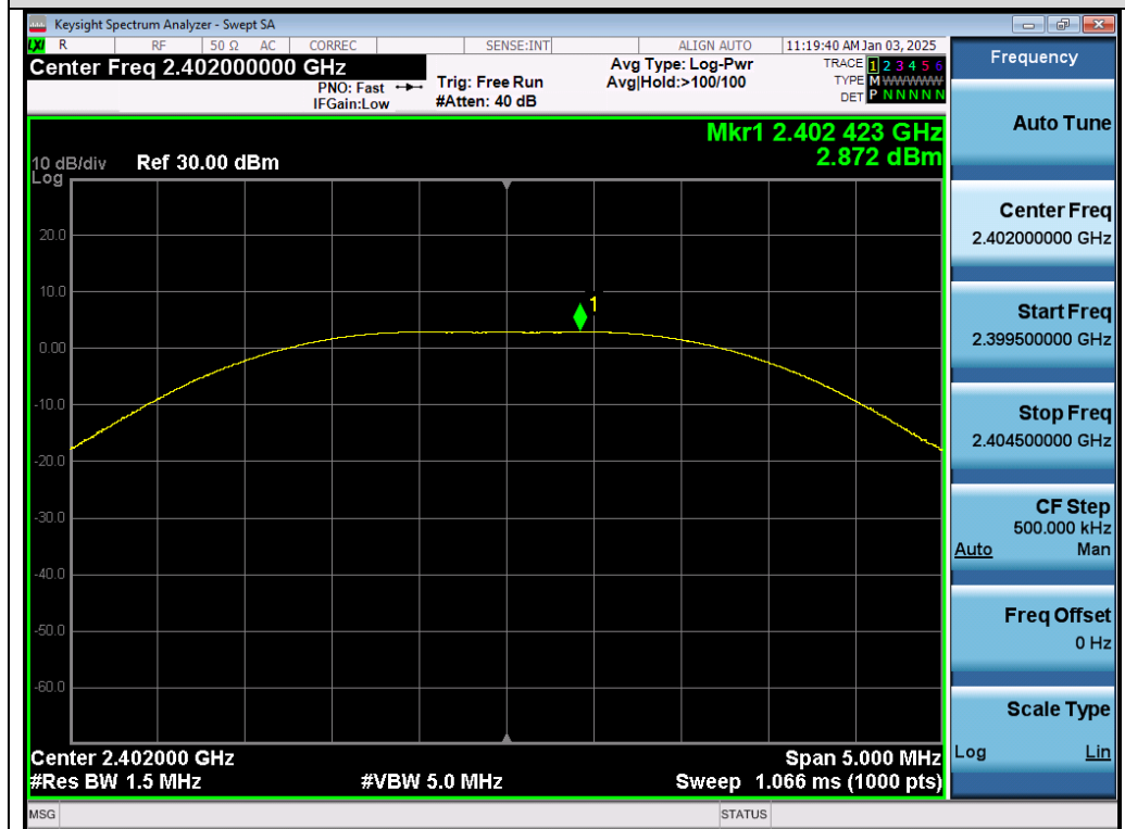
Test_Graph_2.4G_SRD_ANT4_2402_2Mbps_Peak Power
