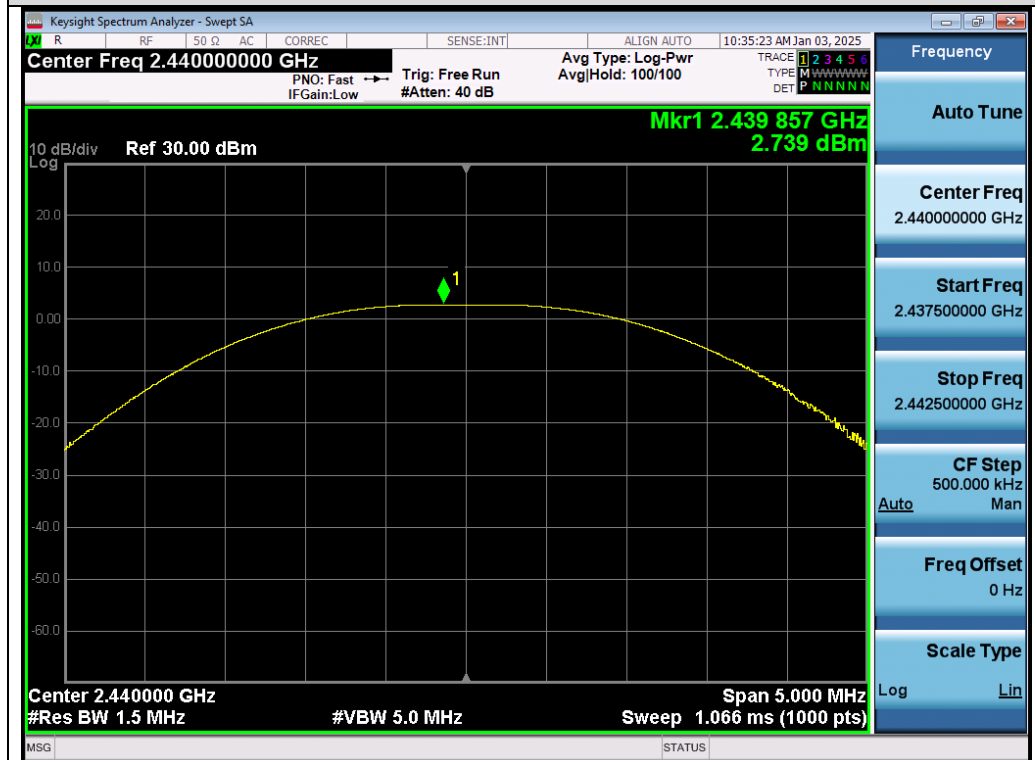
Test_Graph_2.4G_SRD_ANT3_2440_1Mbps_Peak Power
