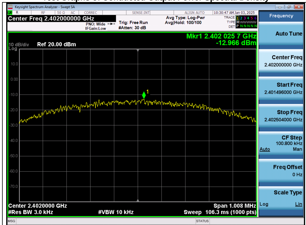
Test_Graph_2.4G_SRD_ANT3_2402_1Mbps_PSD
