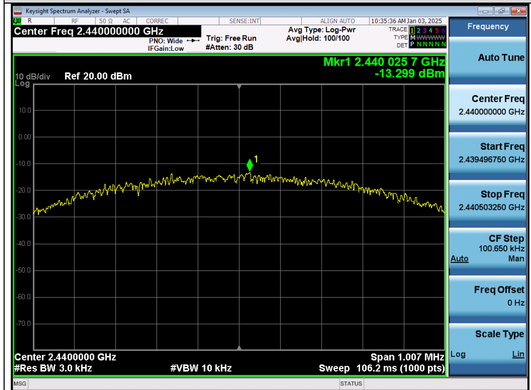
Test_Graph_2.4G_SRD_ANT3_2440_1Mbps_PSD
