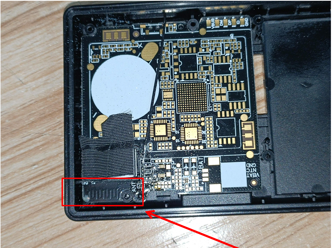
BT Antenna
