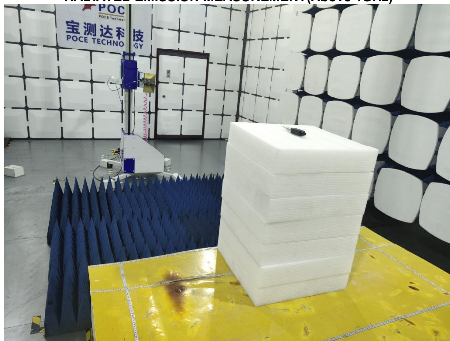
RADIATED EMISSION MEASUREMENT(Above 1GHz)
