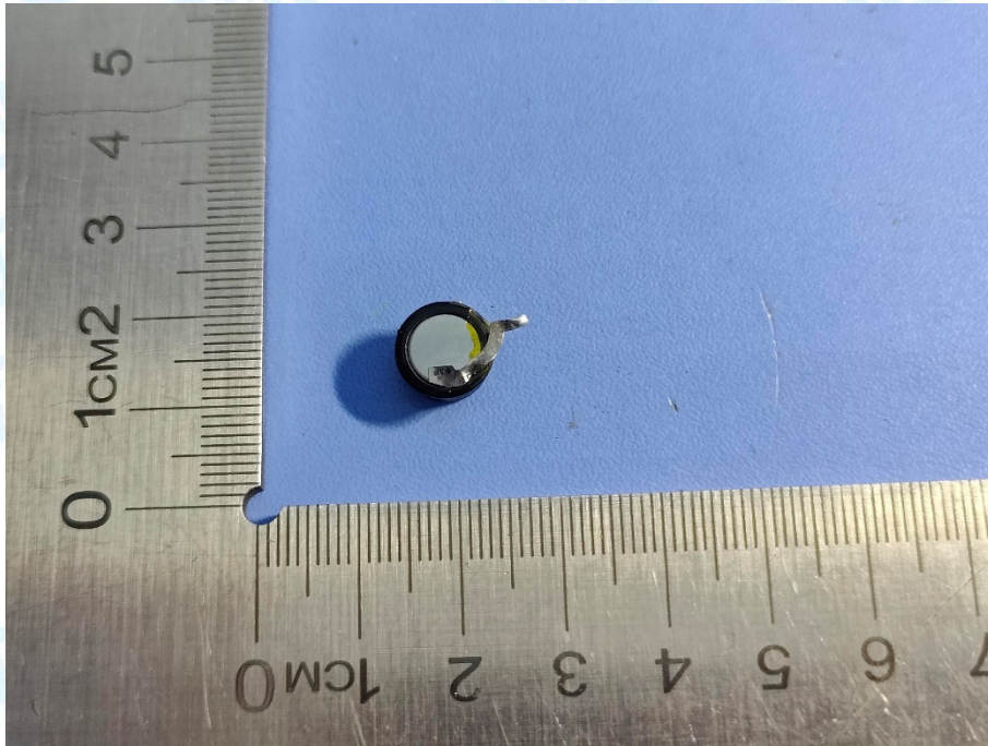
Photo 16 Battery Appearance
