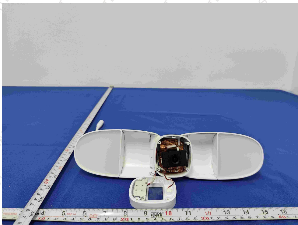
Internal Photograph
