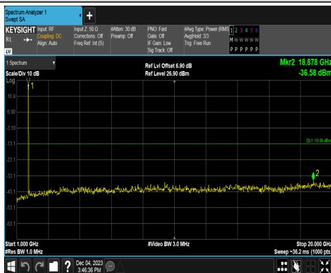
Band4-3MHz-16QAM-19965-1RB#0-Range2:1000~20000MHz
