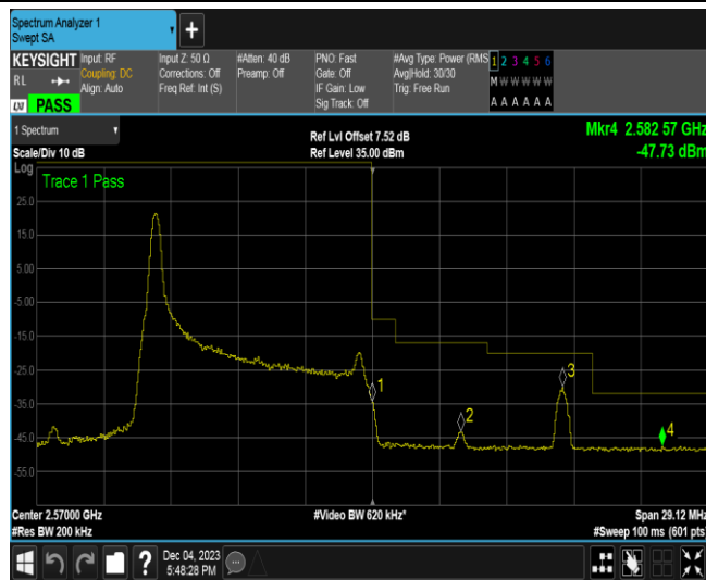
Band7-10MHz-16QAM-21400-1RB#49
