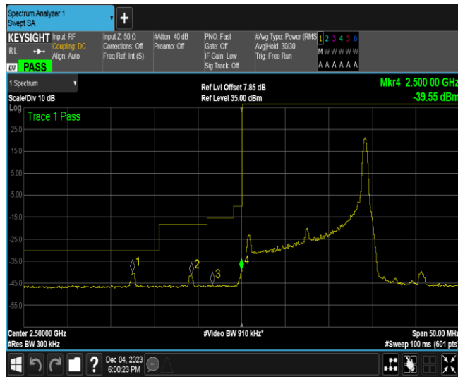
Band7-15MHz-16QAM-20825-75RB#0
