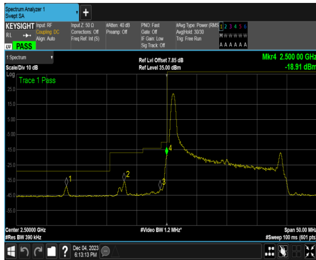
Band7-20MHz-QPSK-20850-1RB#99
