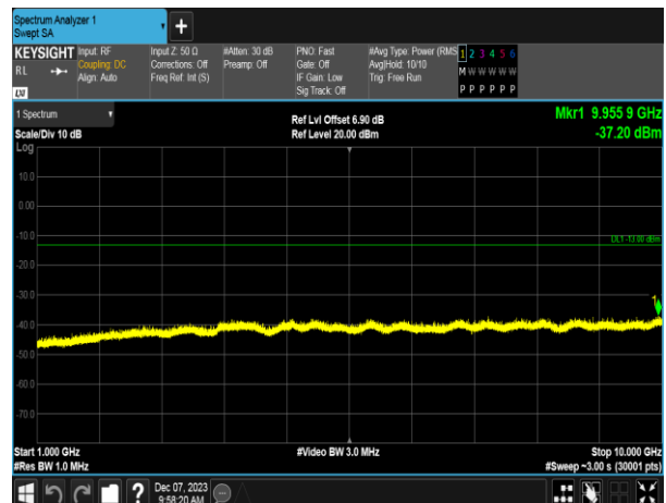
WCDMA 850_HSUPA_MCH
