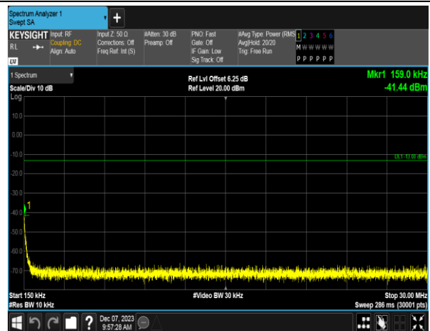
WCDMA 850_HSUPA_MCH
