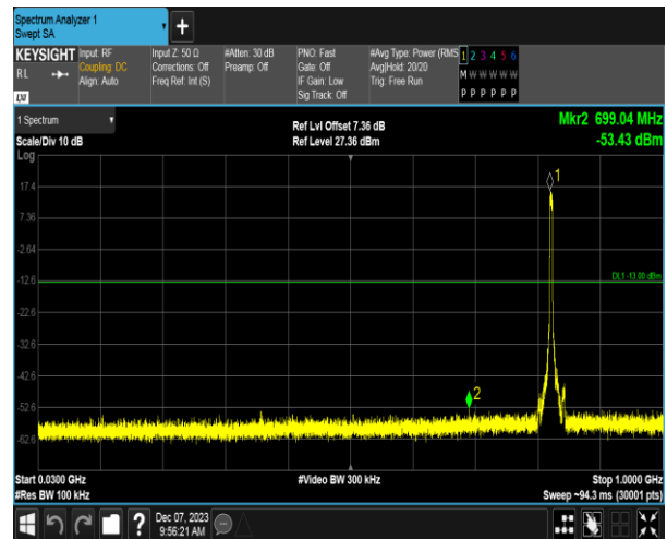
WCDMA 850_HSUPA_MCH
