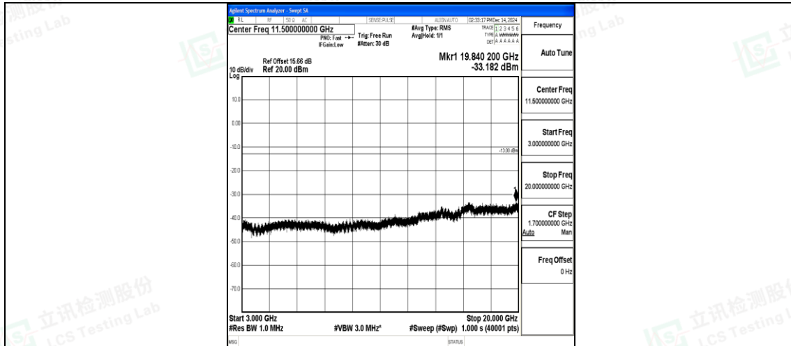
Band2_10MHz_QPSK_18650_1RB#0_3000~20000_3000~20000
