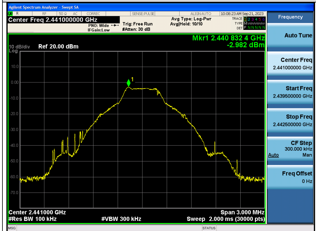
Test Graph BR ANT1 2441 1Mbps Reference Level
