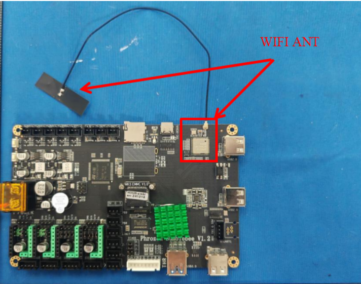
Picture of antenna
