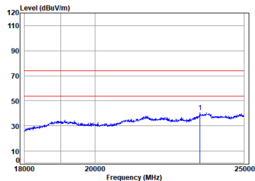
2.4G_SRD_TX_HIGH_Horizontal
