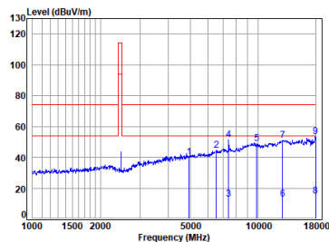
2.4G_SRD_TX_HIGH_Horizontal
