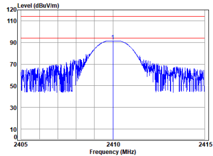
2.4G_SRD_LOW_TX_Vertical
