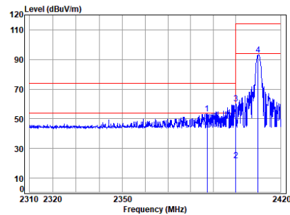
2.4G_SRD_LOW_TX_Vertical
