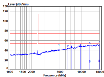
2.4G_SRD_TX_MID_Horizontal
