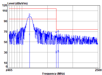
2.4G_SRD_HIGH_TX_Horizontal
