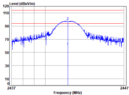
2.4G_SRD_MID_TX_Horizontal
