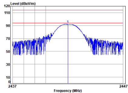
2.4G_SRD_MID_TX_Vertical
