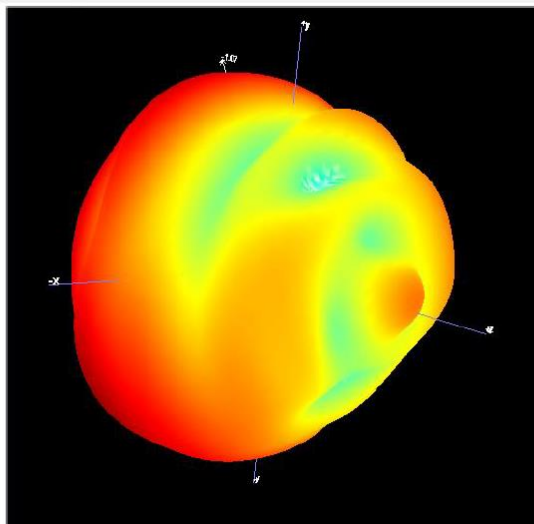
B1.3 3D Pattern for 2500MHz
