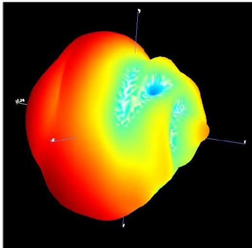
B1.2 3D Pattern for 2450MHz
