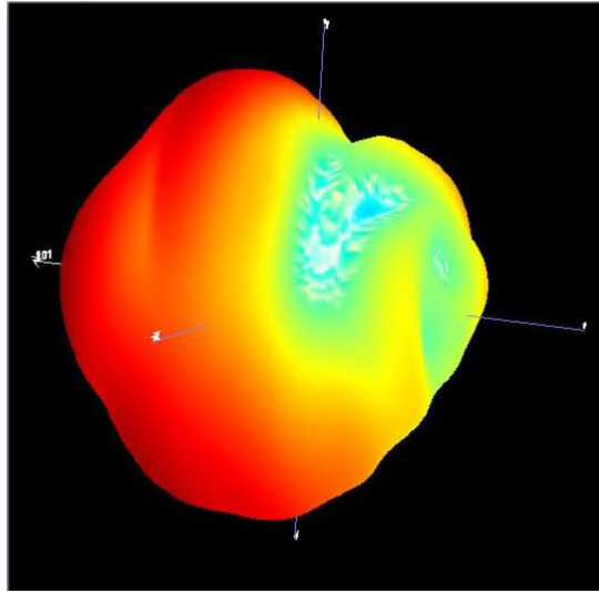
B1.1 3D Pattern for 2400MHz
