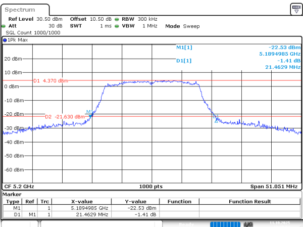
802.11a_5200MHz_Chain 0
