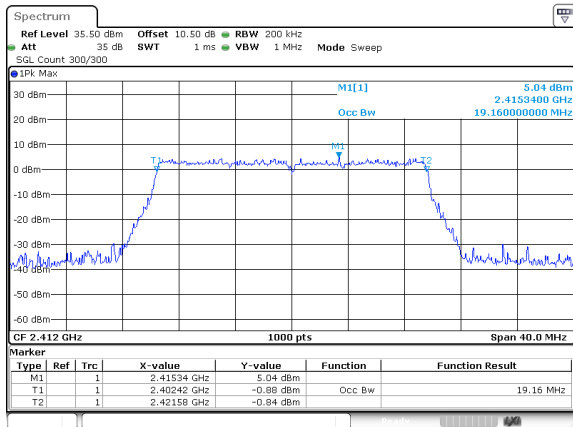
802.11ax20_2412MHz_RU_FULL_Chain 0
