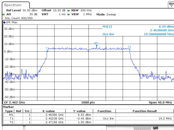
802.11ax20_2462MHz_RU_FULL_Chain 0
