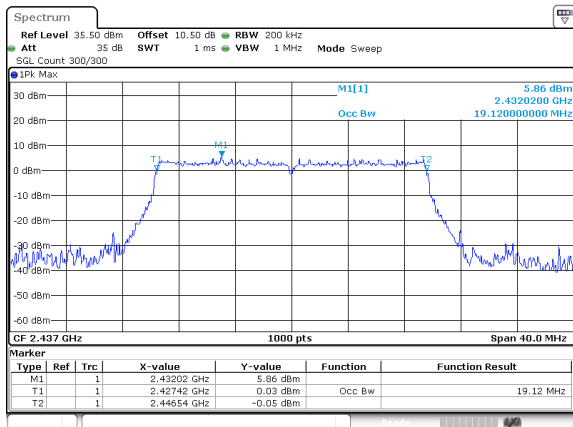
802.11ax20_2437MHz_RU_FULL_Chain 1
