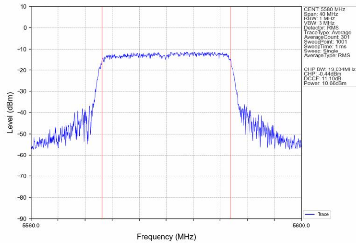
802.11ax(HEW20)_MCH_5580MHz_SU_/_Ant1_NTNV
