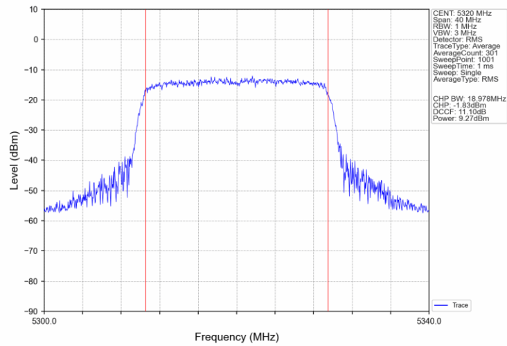
802.11ax(HEW20)_HCH_5320MHz_SU_/_Ant1_NTNV
