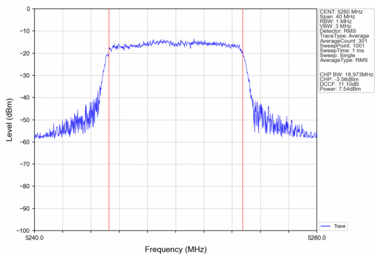
802.11ax(HEW20)_LCH_5260MHz_SU_/_Ant1_NTNV
