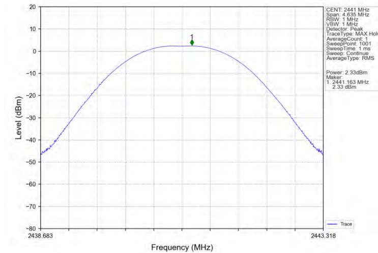
GFSK_DH5_MCH_2441MHz_Ant1_NTNV
