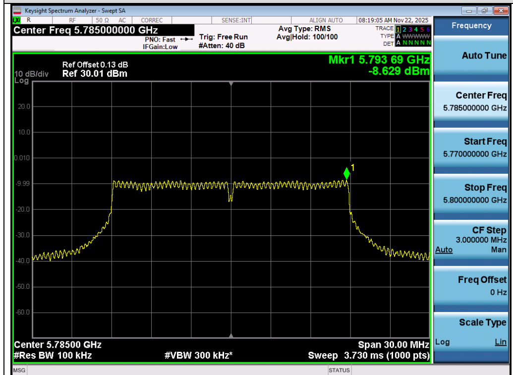
Test_Graph_802.11n20_ANT1_5785_MCS0_PSD
