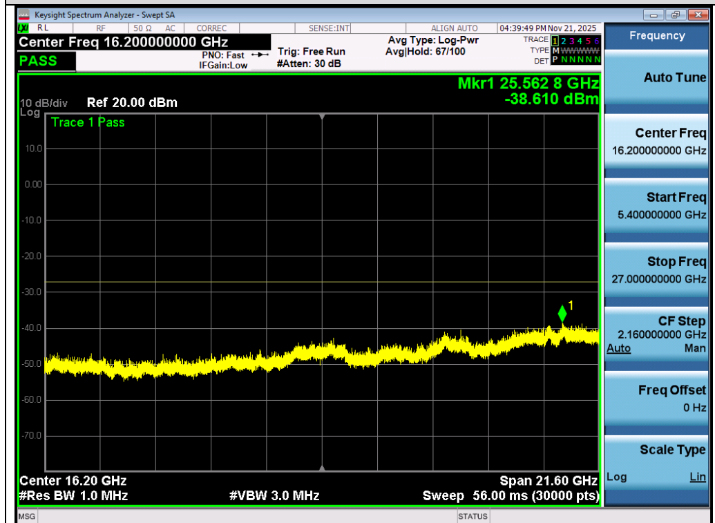
Test_Graph_802.11n40_ANT1_5270_MCS0_Frequency Band 4
