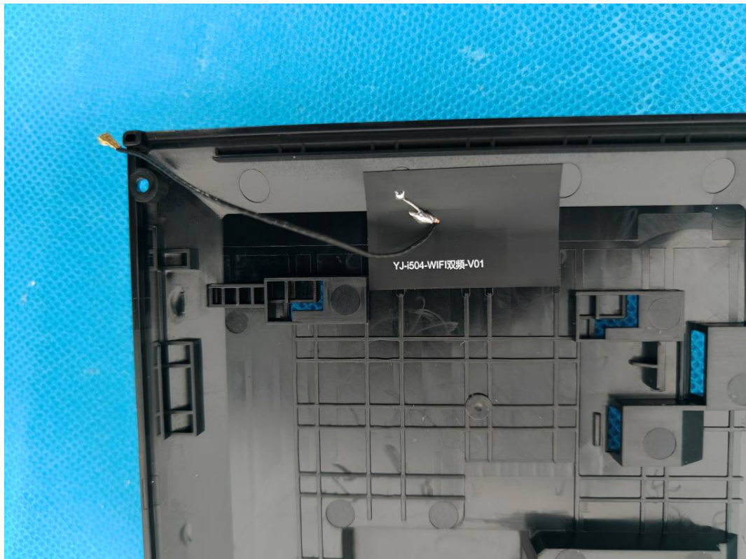
WiFi ANT
