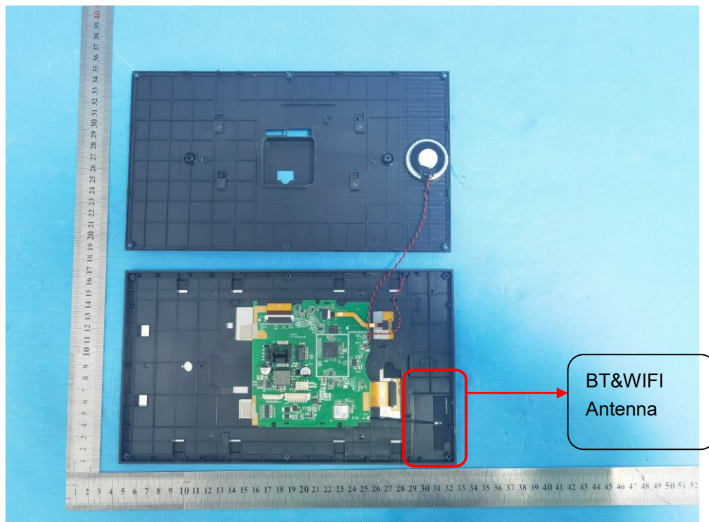
Series Model: i556W Open View-1 of EUT
