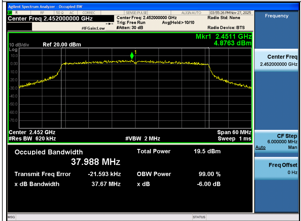
Test_Graph_802.11ax40_ANT2_2452_MCS0_DTSBW
