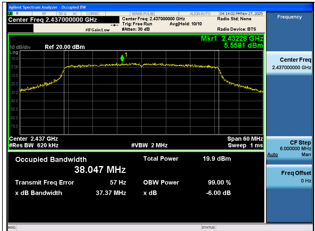
Test_Graph_802.11ax40_ANT2_2437_MCS0_DTSBW
