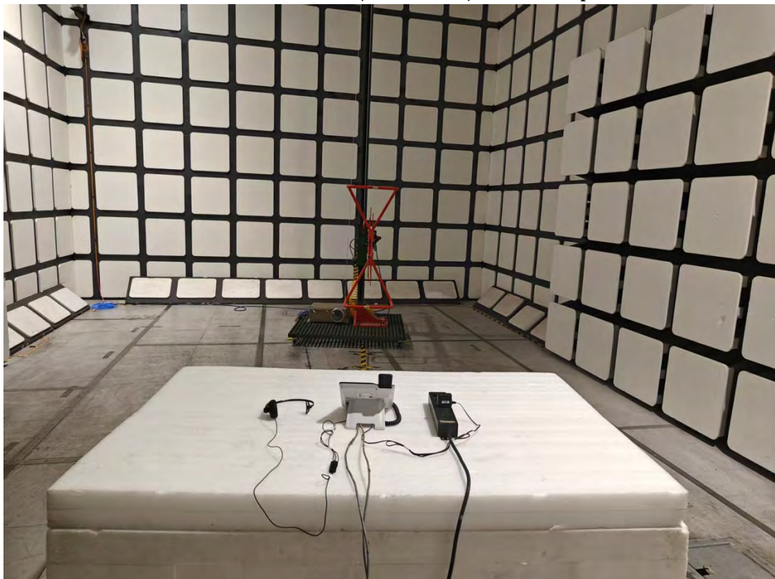
Radiated Emissions View (Below 1 GHz)_J600W_Adapter 2
