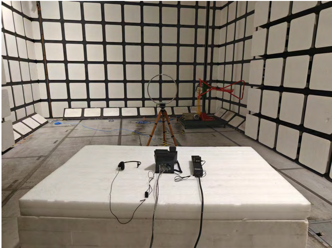
Radiated Emissions View (Below 30MHz)_X303W_Adapter 2
