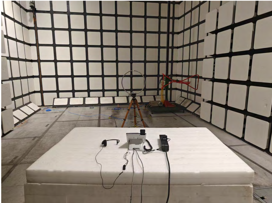
Radiated Emissions View (Below 30MHz)_J600W_Adapter 2
