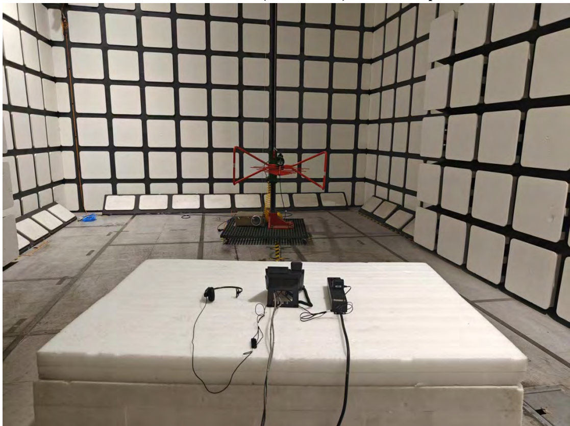
Radiated Emissions View (Below 1 GHz)_X303W_Adapter 2
