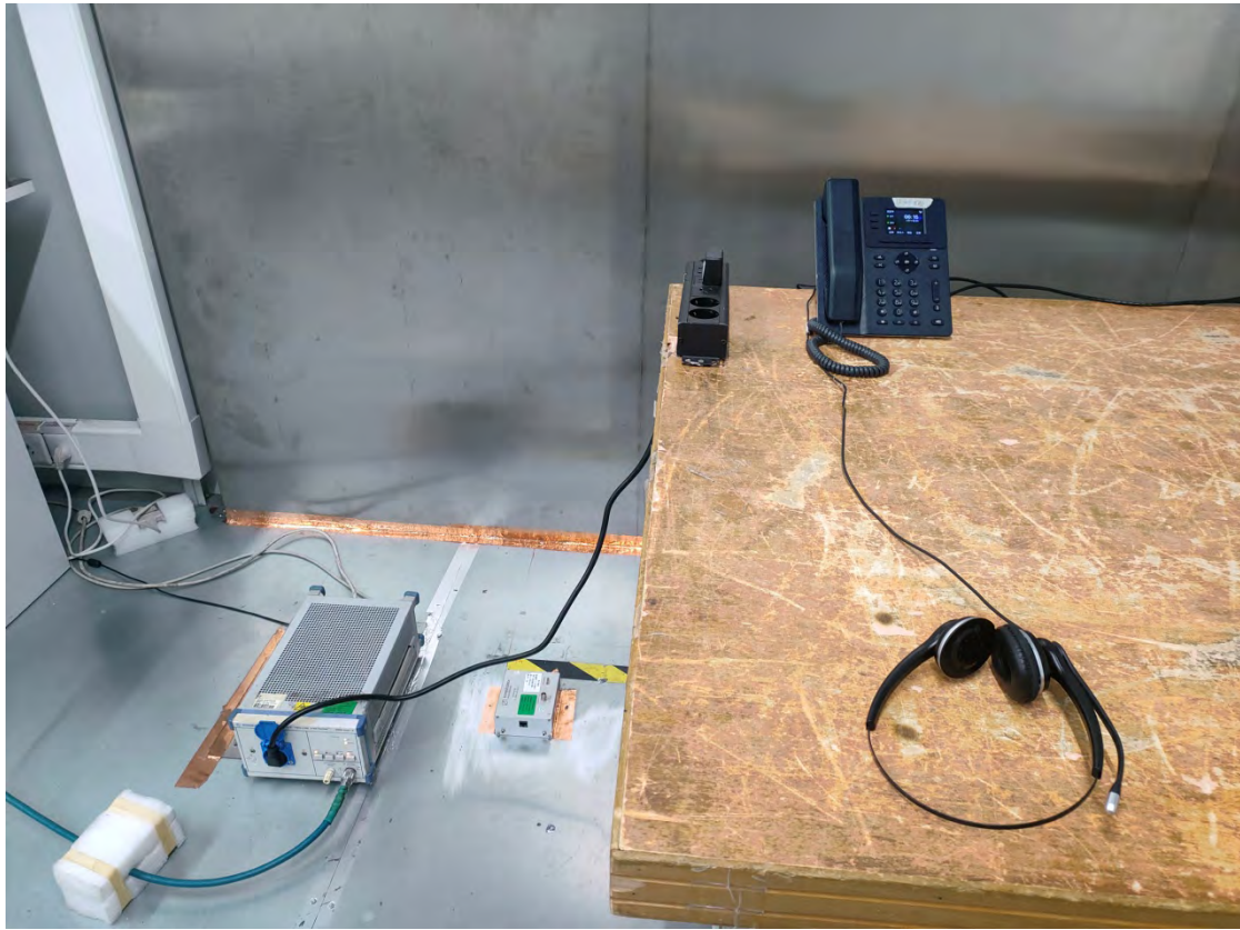
Conducted Emissions - Front View_J600W_Adapter 2
