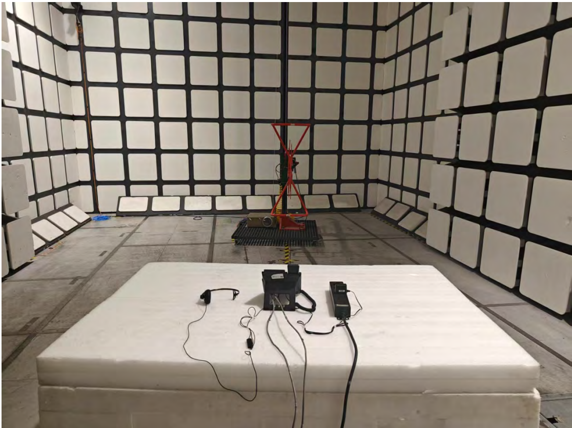
Radiated Emissions View (Below 1 GHz)_J303W_Adapter 2
