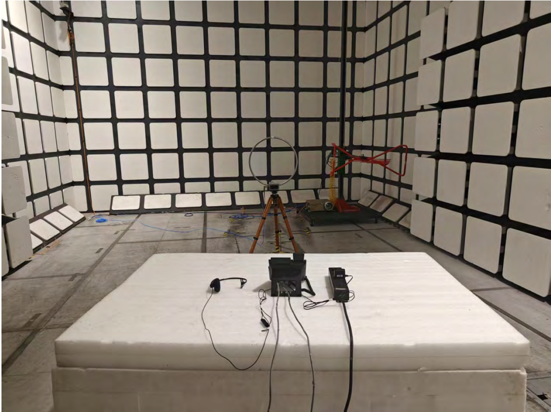
Radiated Emissions View (Below 30MHz)_J303W_Adapter 2
