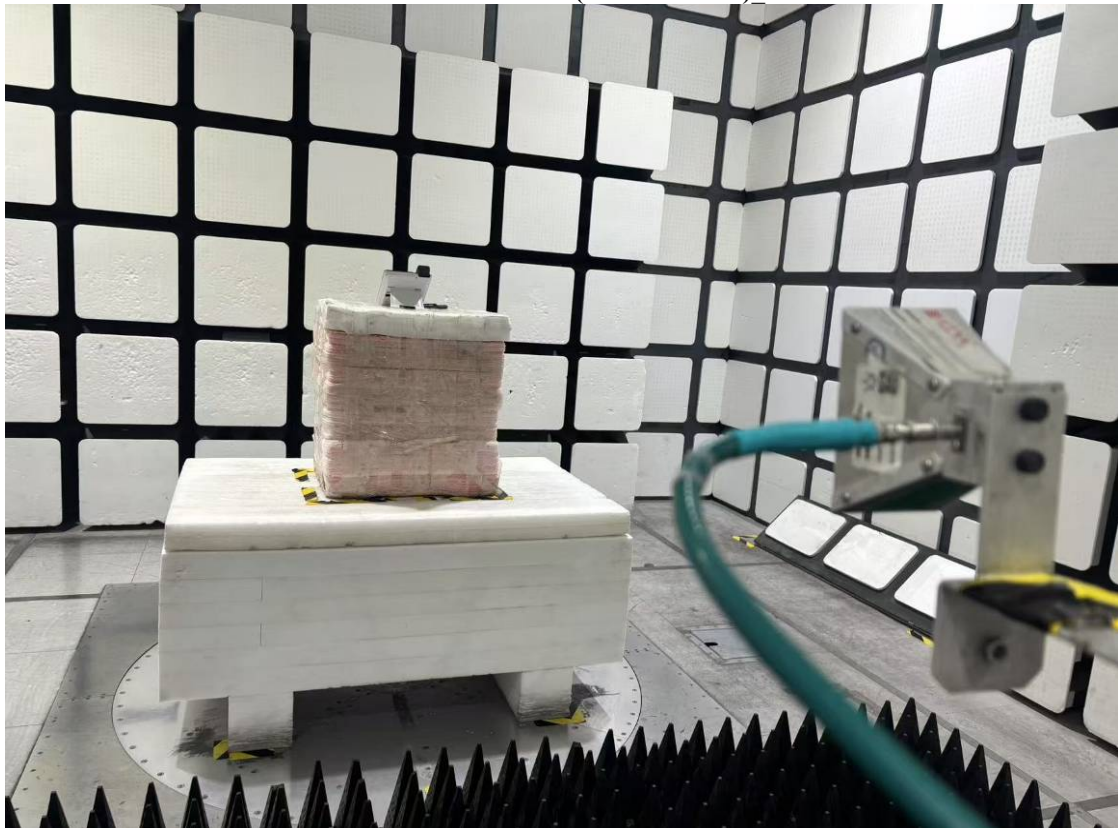
Radiated Emissions View (Above 18GHz) J600W
