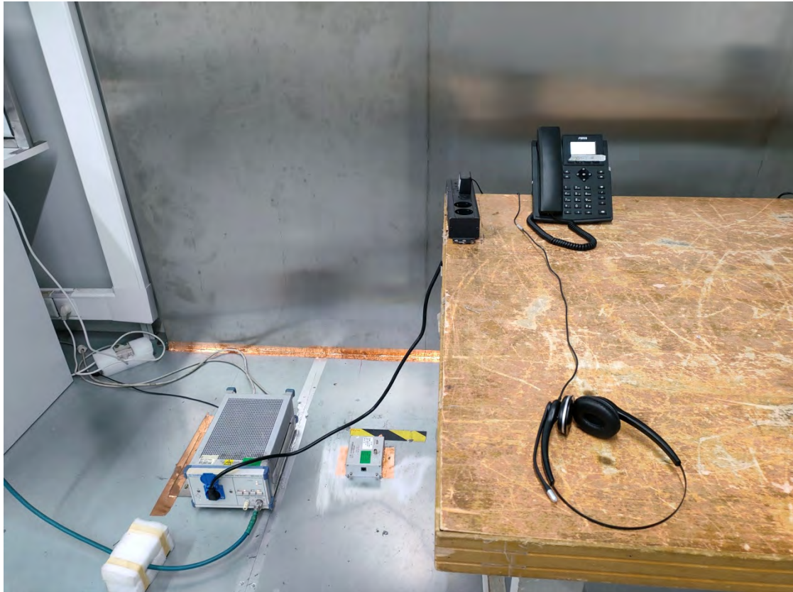
Conducted Emissions - Front View_X301W_Adapter 2
