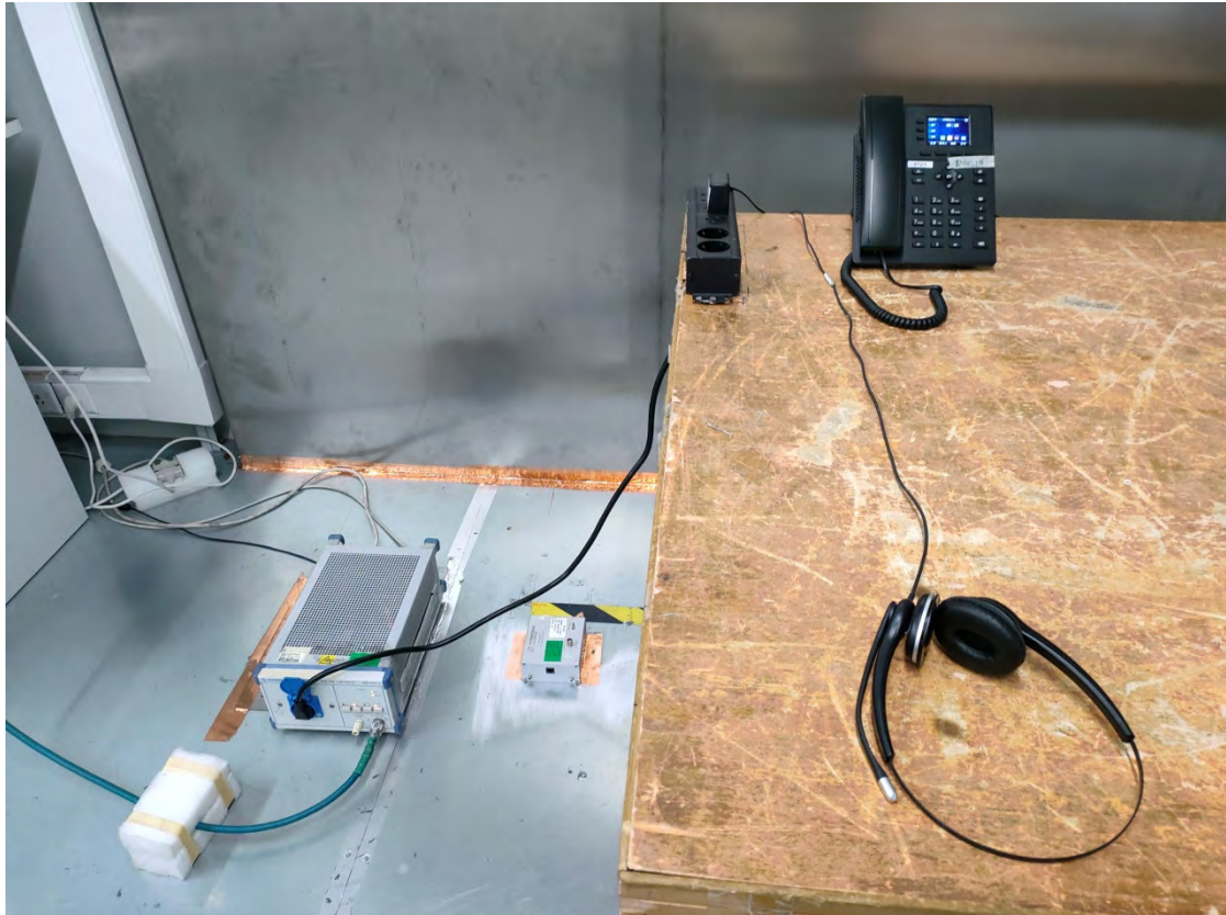
Conducted Emissions - Front View_X303W_Adapter 2
