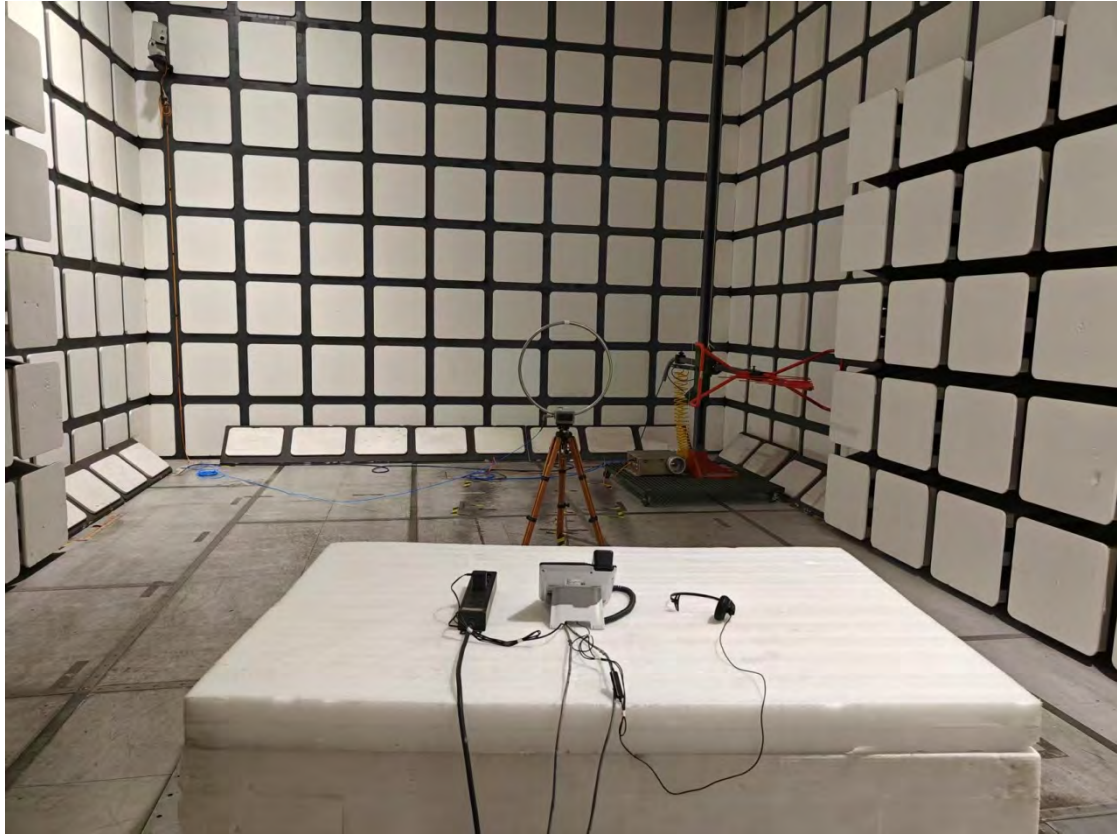
Radiated Emissions View (Below 30MHz)_J600W_Adapter 1
