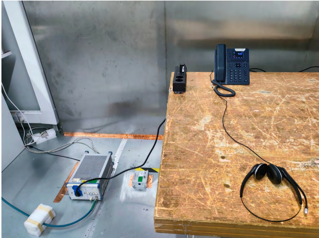
Conducted Emissions - Front View_J600W_Adapter 1
