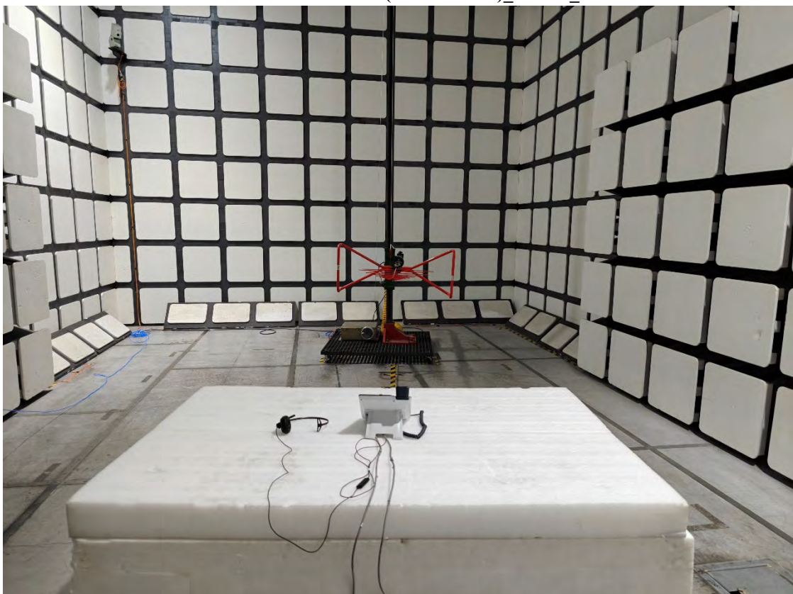
Radiated Emissions View (Below 1 GHz)_J600W_POE
