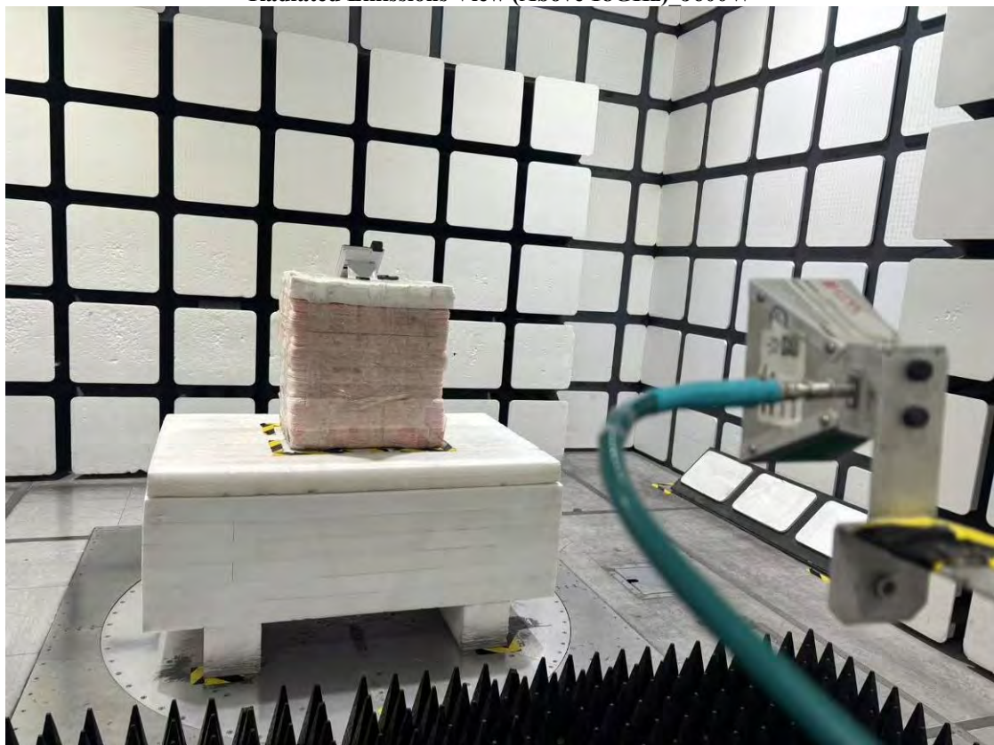
Radiated Emissions View (Above 18GHz) J600W
