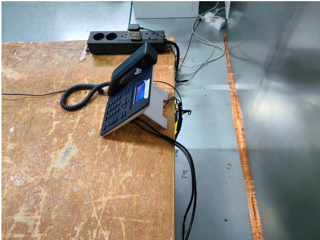
Conducted Emissions - Side View_J600W_Adapter 1
