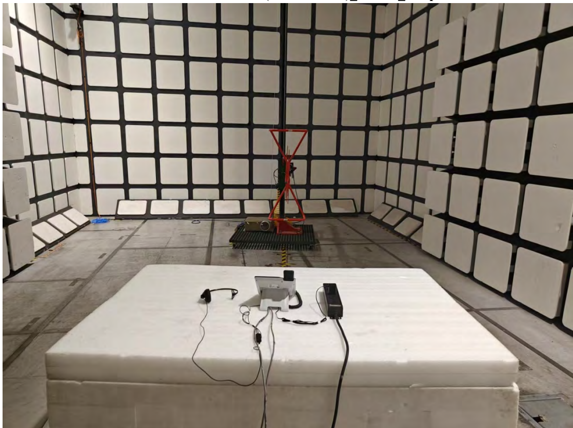
Radiated Emissions View (Below 1 GHz)_J600W_Adapter 1
