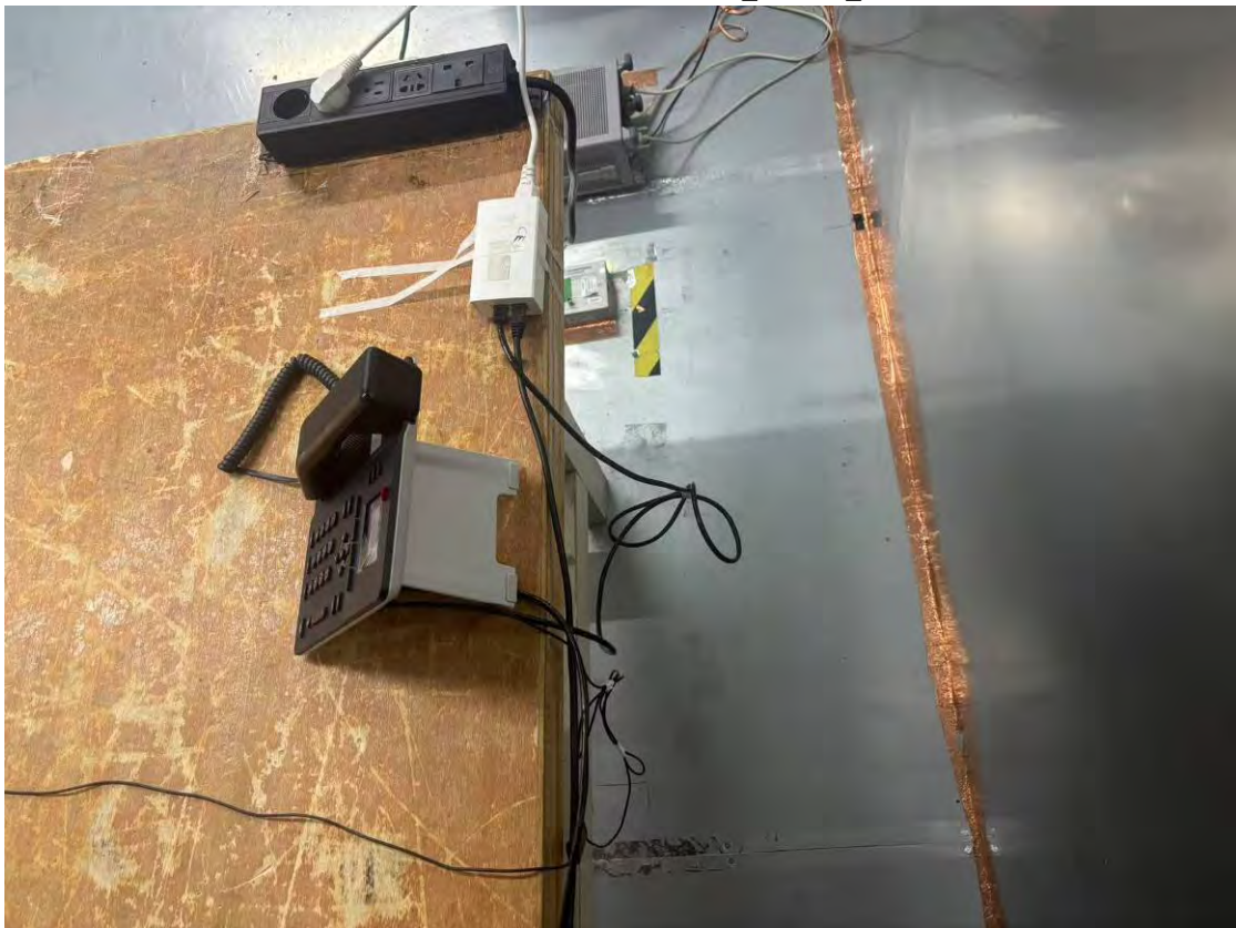
Conducted Emissions - Side View_J600W_POE
