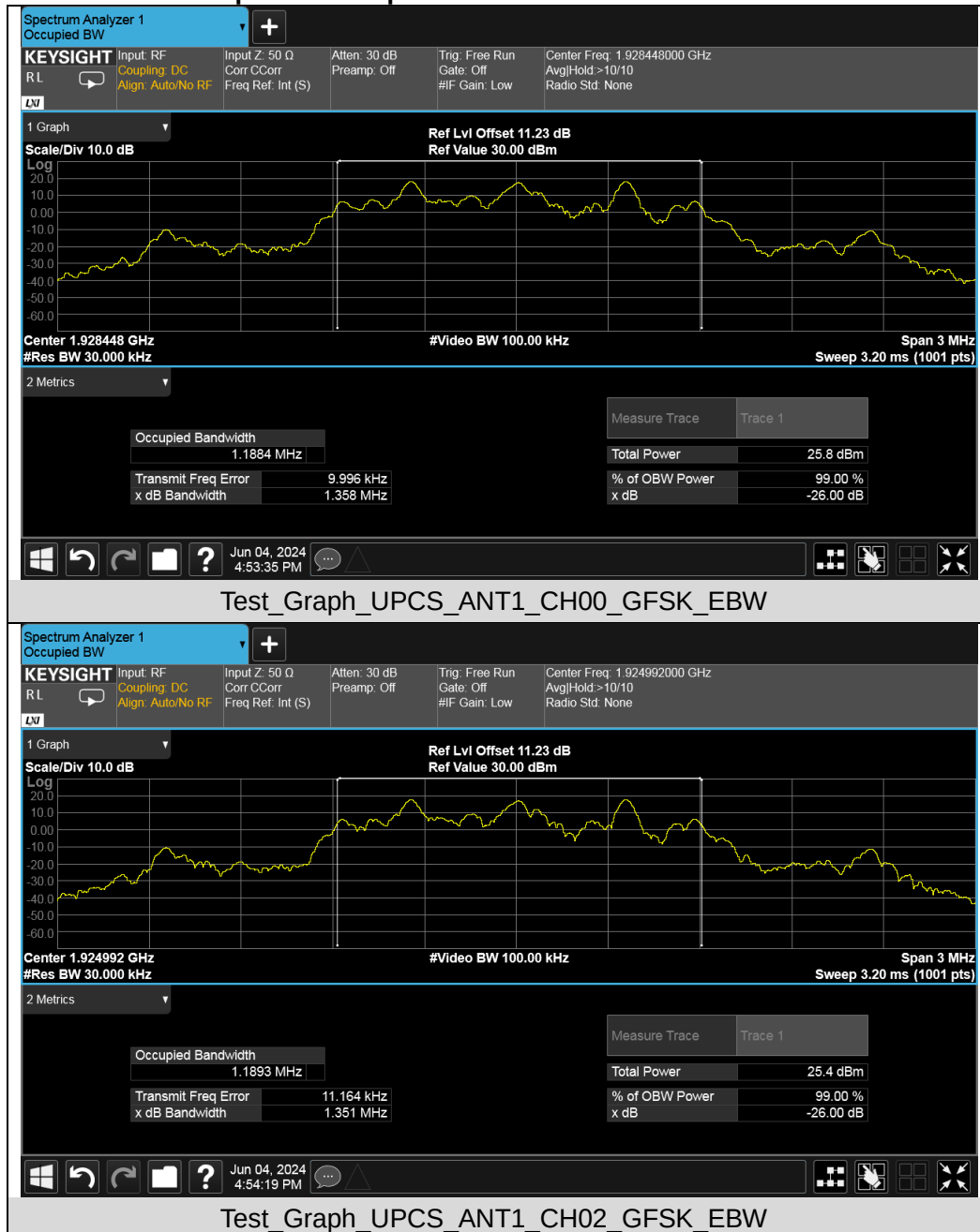
Test Graphs of Occupied Bandwidth and -26dB Bandwidth
