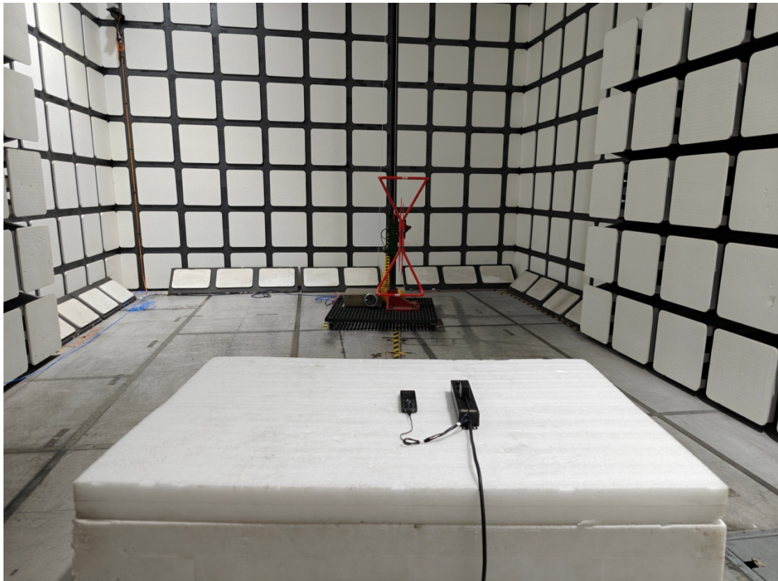
Radiated Emissions View (Below 1GHz) _ Adapter 2
