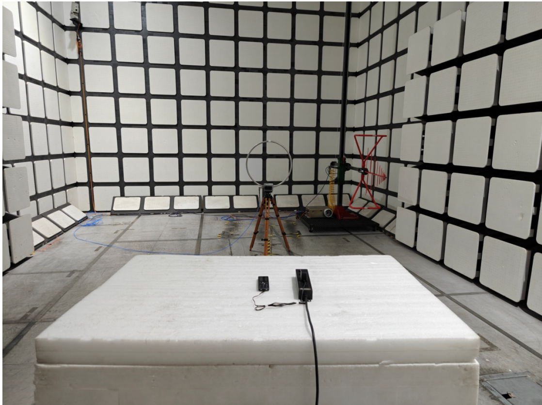
Radiated Emissions View (Below 30MHz) _ Adapter 1
