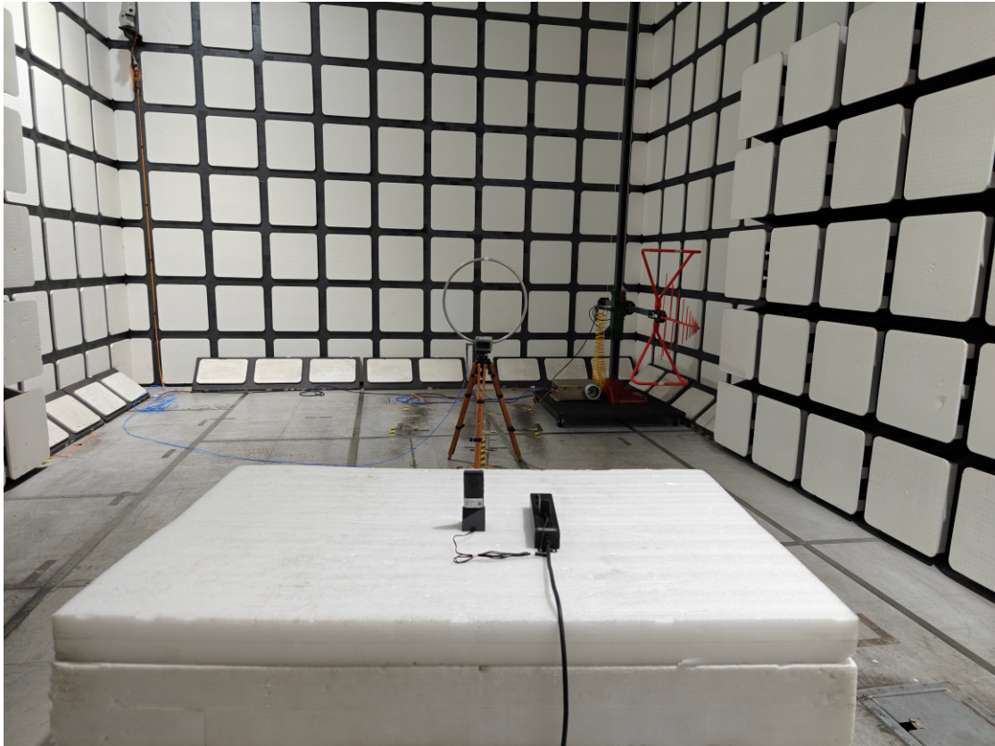
Radiated Emissions View (Below 30MHz) _ Adapter 1 +Charger
