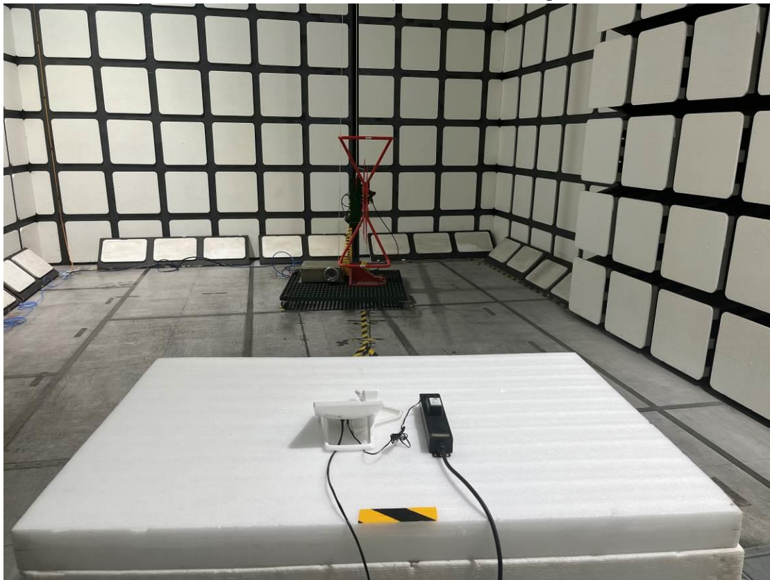
Radiated Emissions View (Below 1 GHz)_Adapter 1
