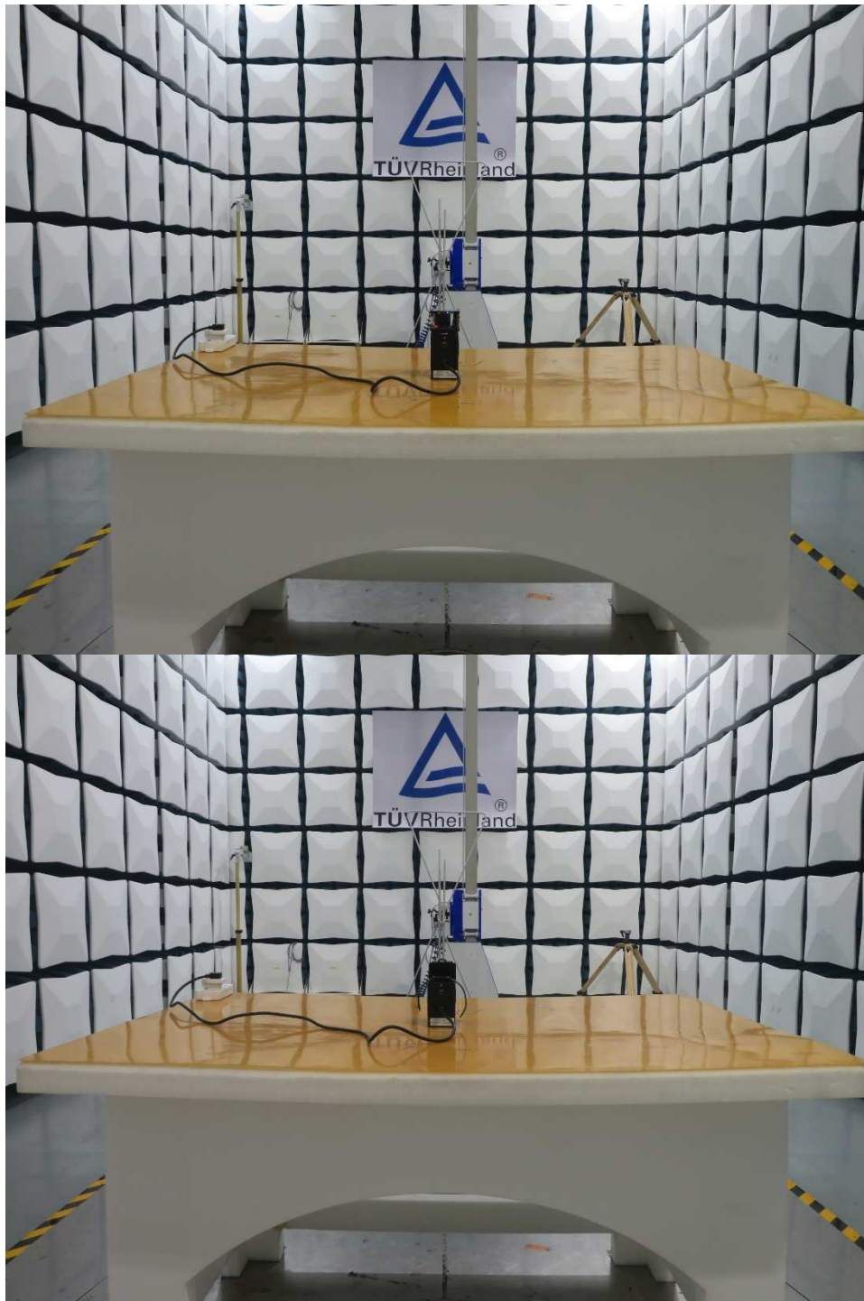
Photograph 2: Set-up photo for Radiated Spurious Emission, 30MHz - 1GHz
