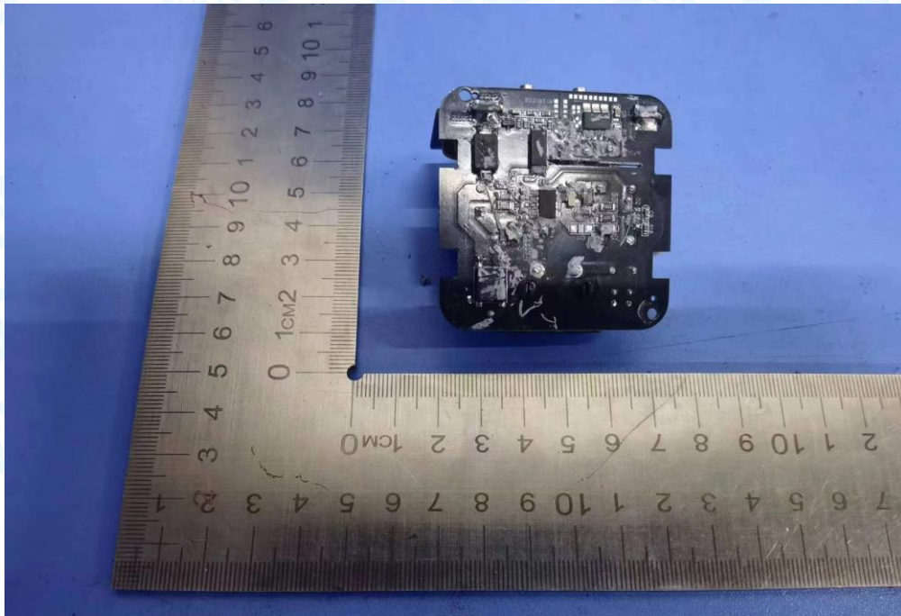
Photo 17 Appearance of PCB
