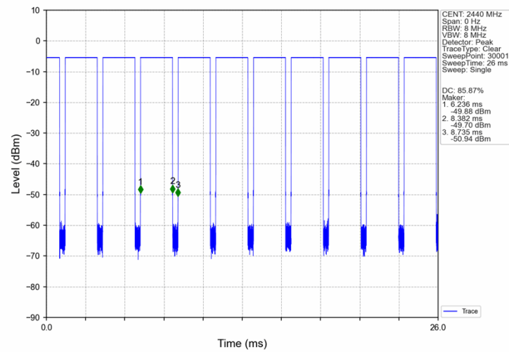
1M_MCH_2440MHz_Ant1_NTNV
