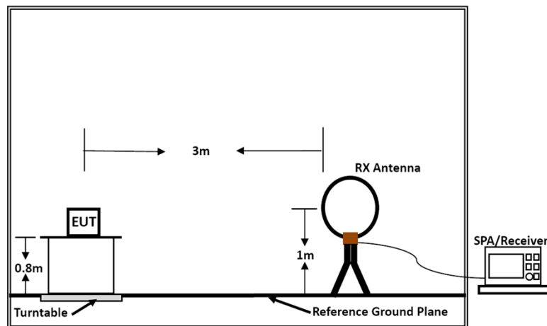
Below 30MHz
