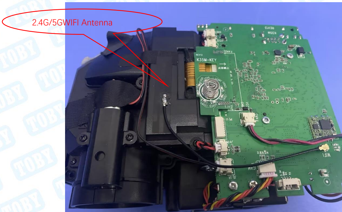
Photo 15 Appearance of PCB
