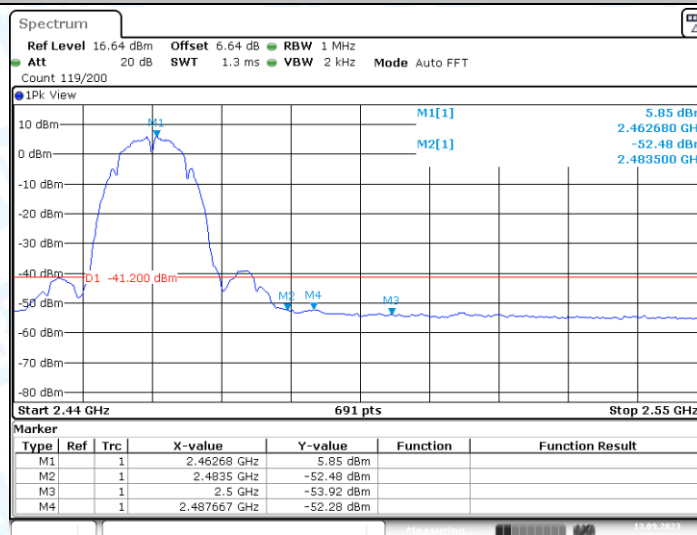
11B_Ant1_High_2462_AV
