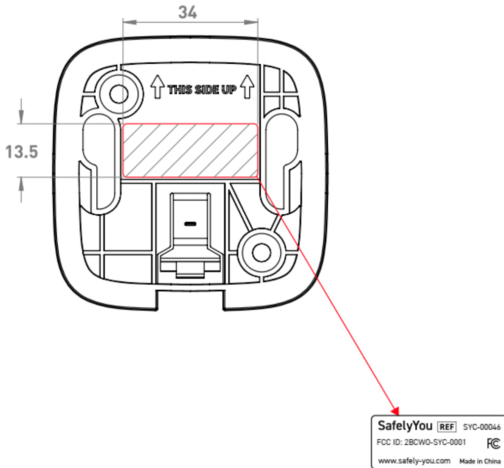
Figure 1 – Halo™ Wall Button
