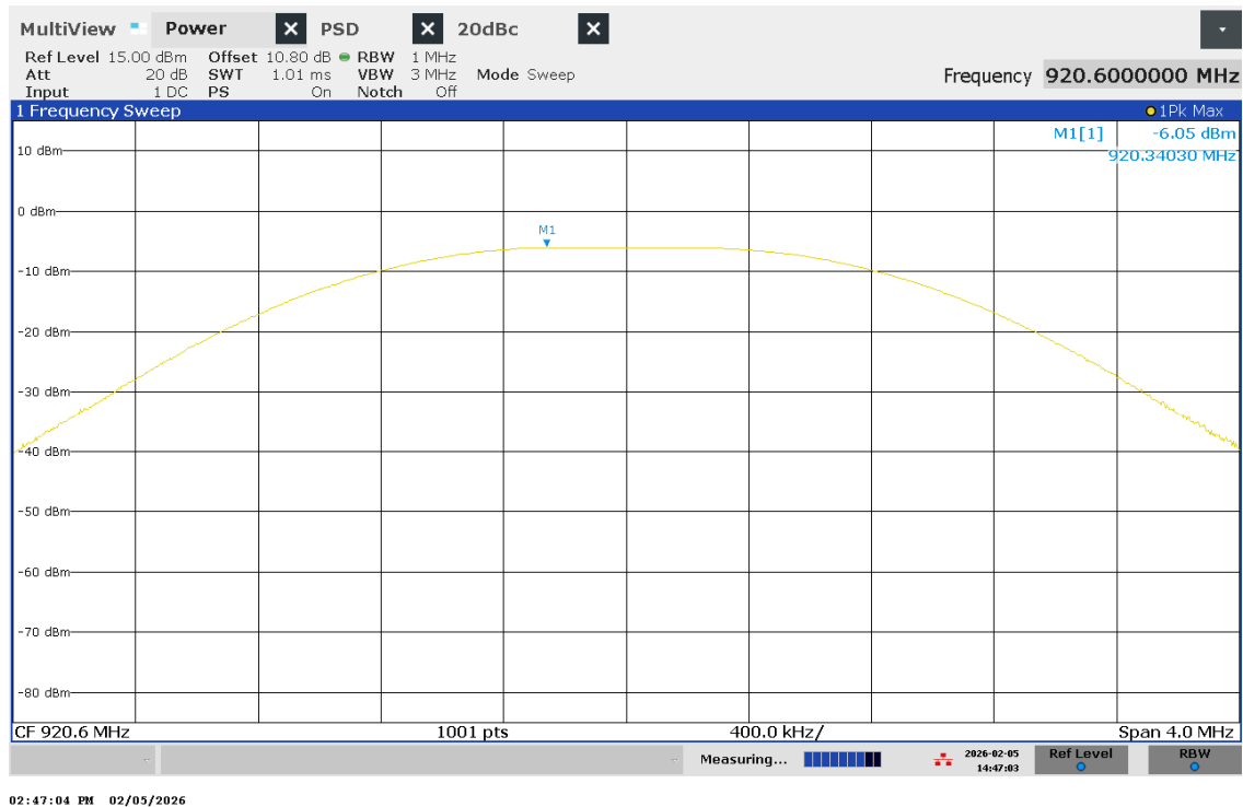
Figure 14 – Peak Power – Channel 12
