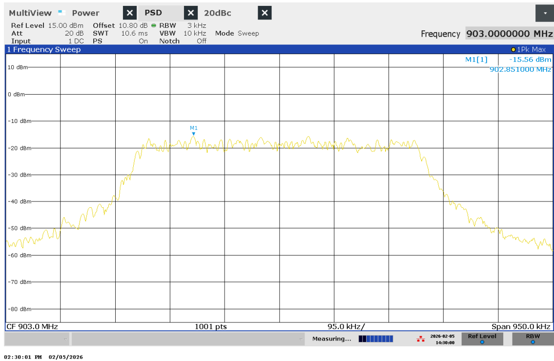
Figure 20 – PSD – Channel 1
