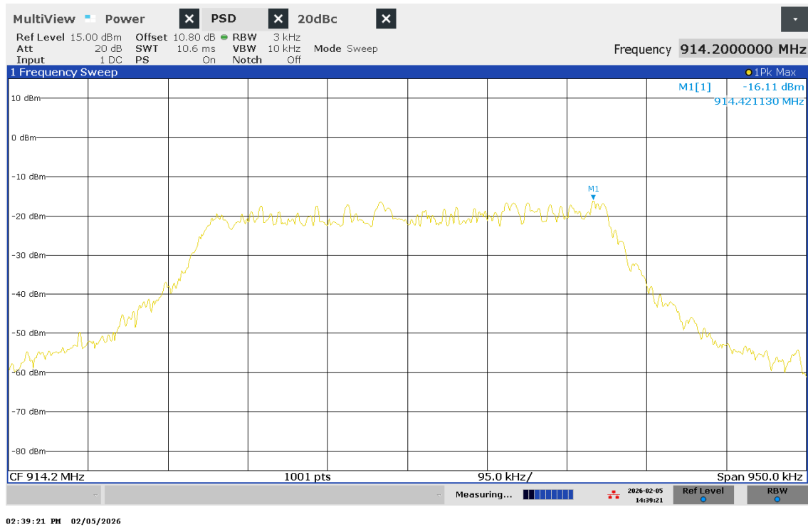
Figure 22 – PSD – Channel 8
