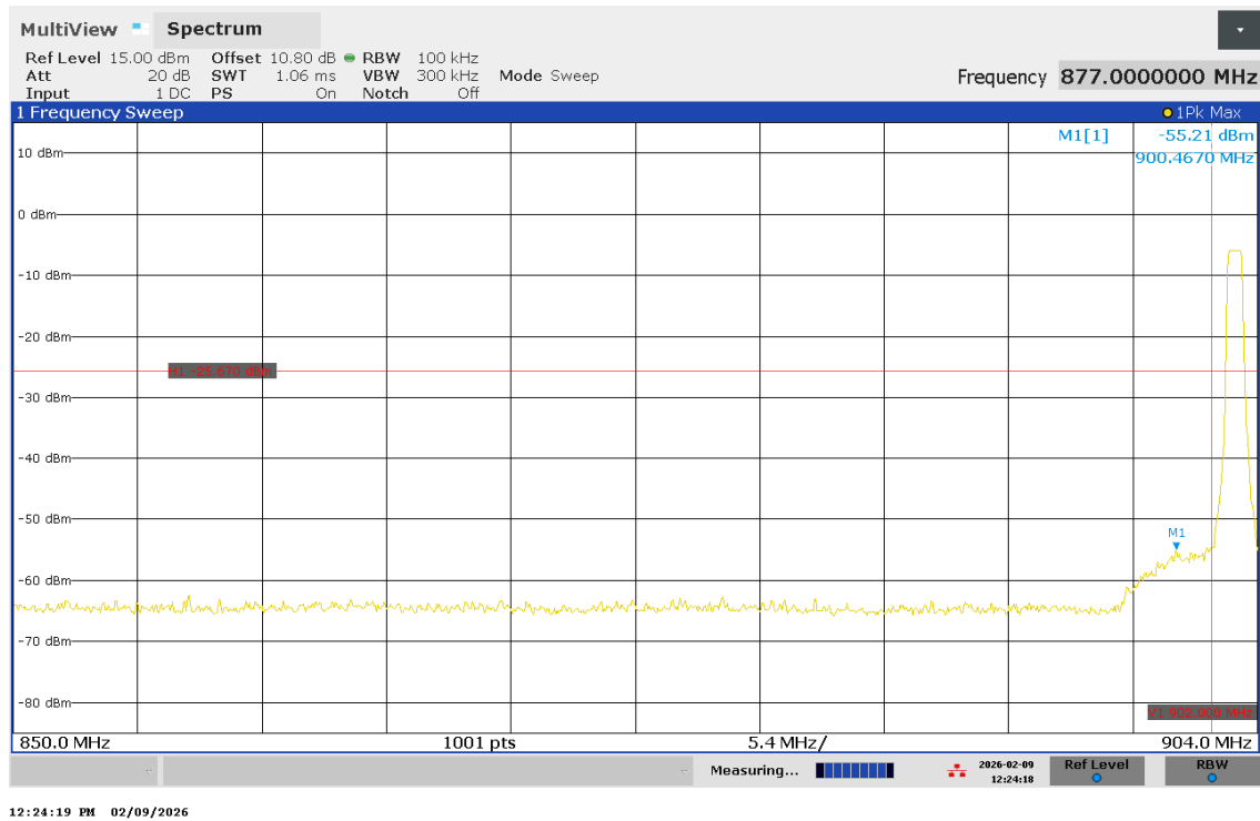
Figure 18 – -20dBc Band Edge – Channel 1
