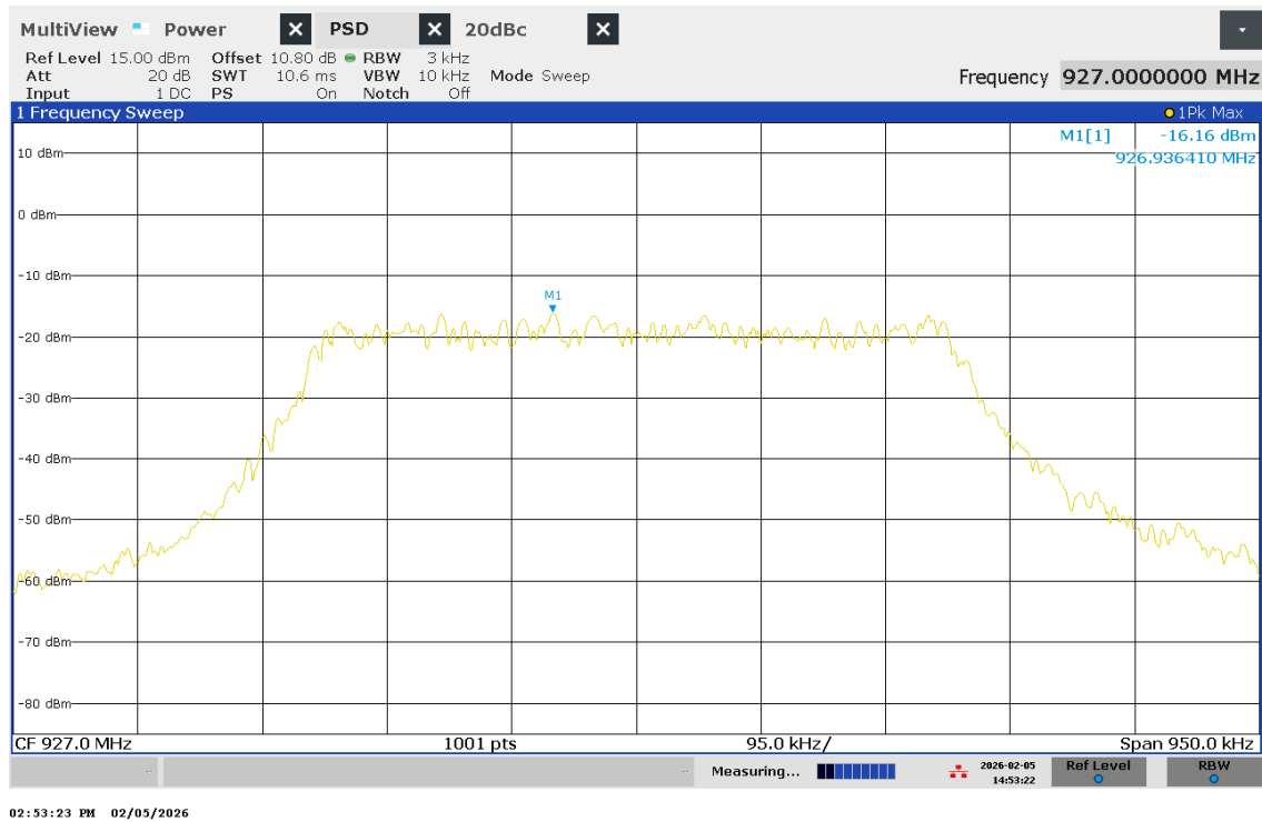
Figure 24 – PSD – Channel 16
