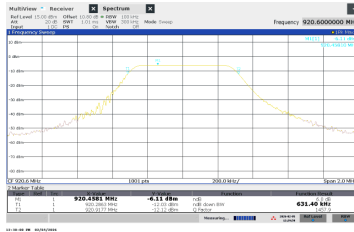
Figure 4 – 6dB Bandwidth – Channel 12
