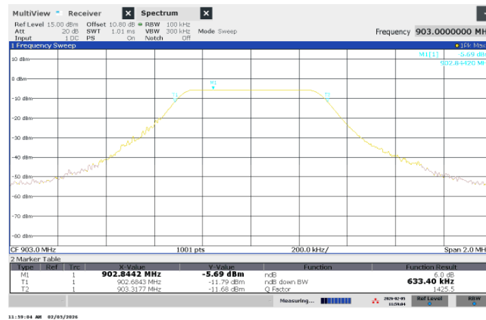
Figure 1 – 6dB Bandwidth – Channel 1
