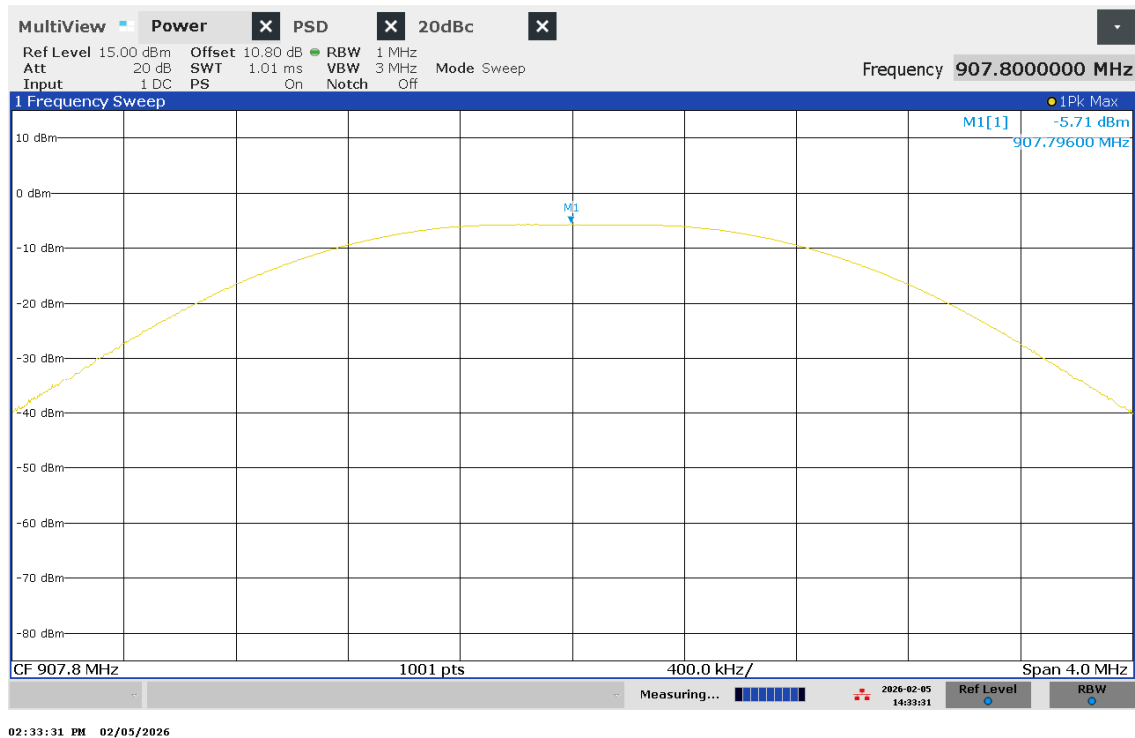
Figure 12 – Peak Power – Channel 4
