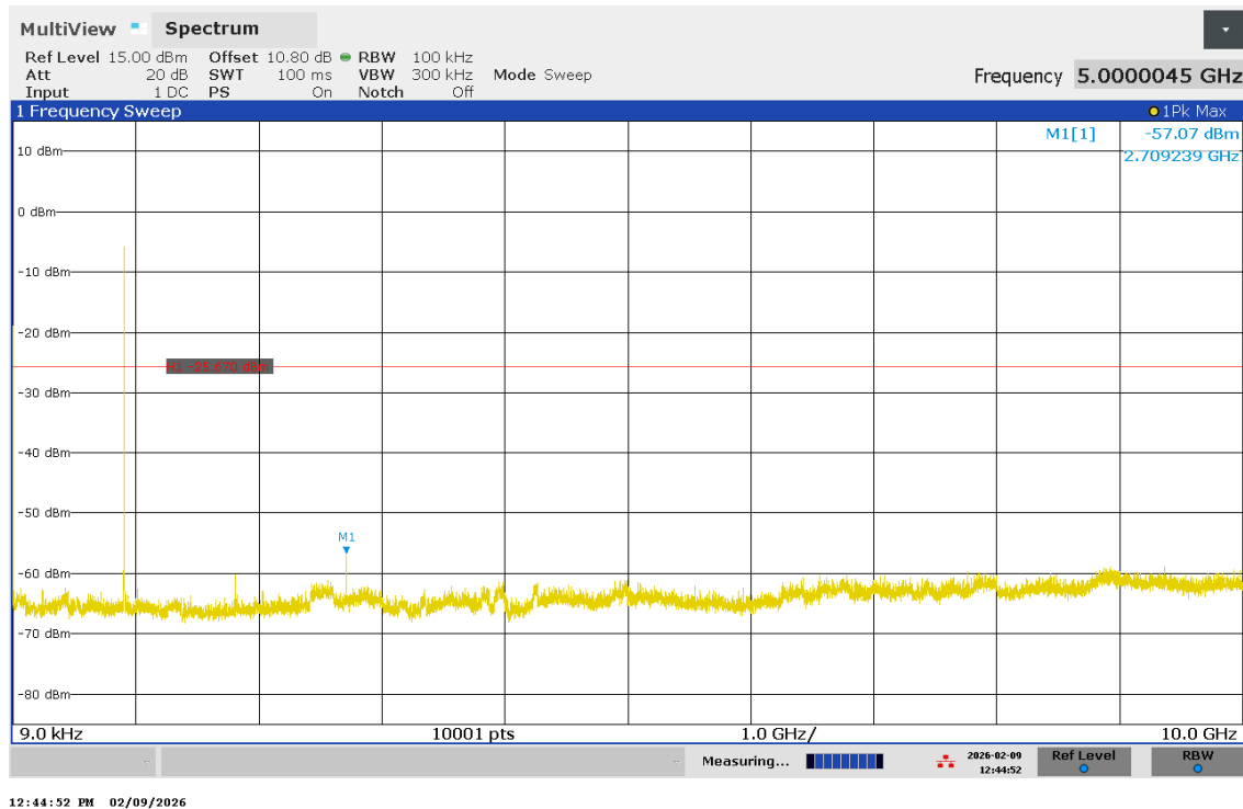
Figure 17 – -20dBc – Channel 1
