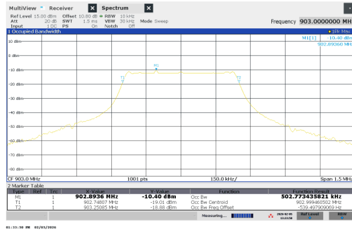
Figure 6 – 99% Bandwidth – Channel 1
