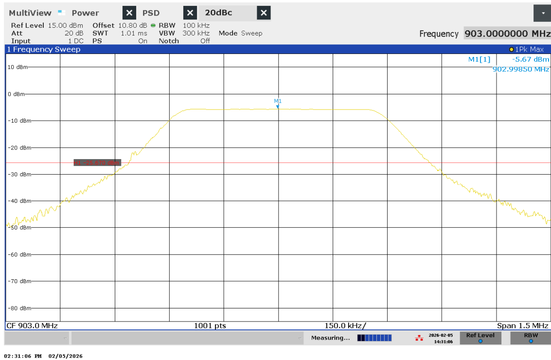
Figure 16 – -20dBc Reference Level – Channel 1
