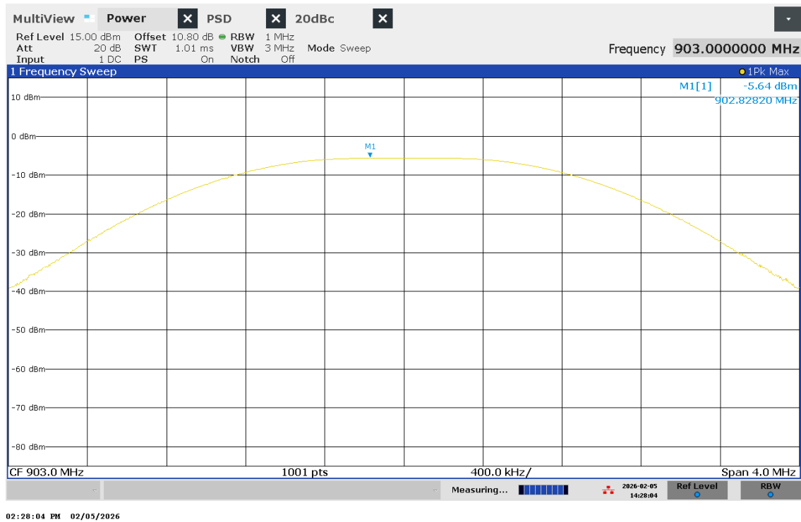
Figure 11 – Peak Power – Channel 1
