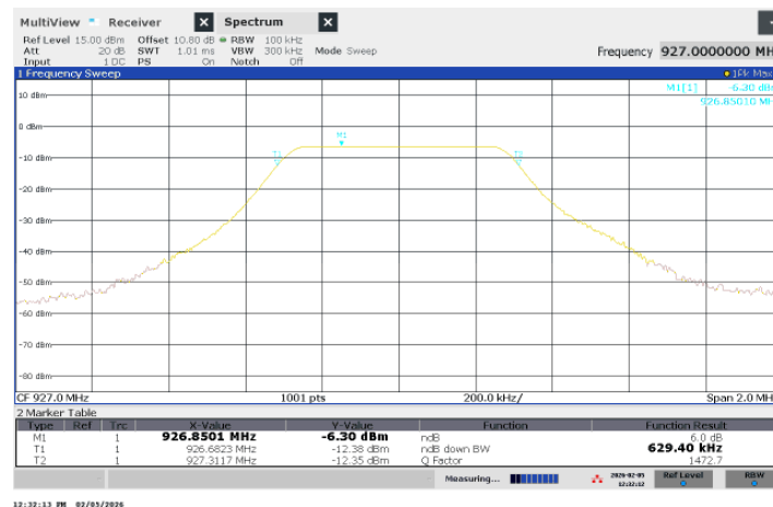
Figure 5 – 6dB Bandwidth – Channel 16
