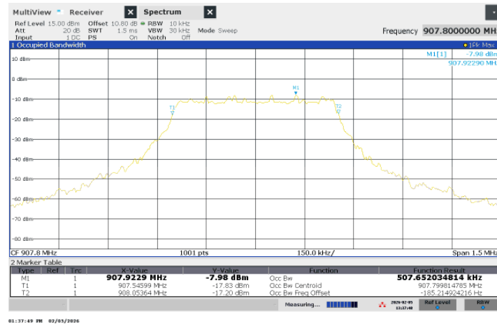
Figure 7 – 99% Bandwidth – Channel 4
