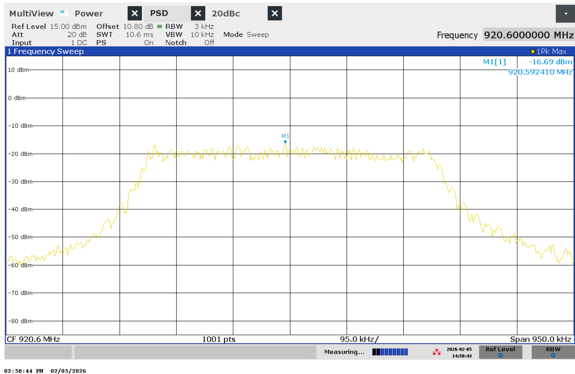
Figure 23 – PSD – Channel 12
