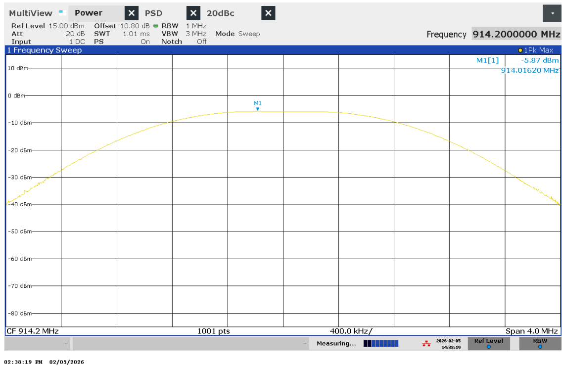
Figure 13 – Peak Power – Channel 8
