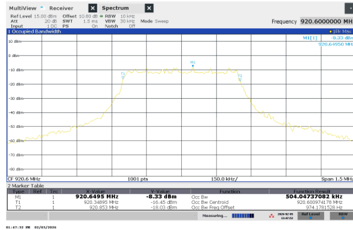
Figure 9 – 99% Bandwidth – Channel 12
