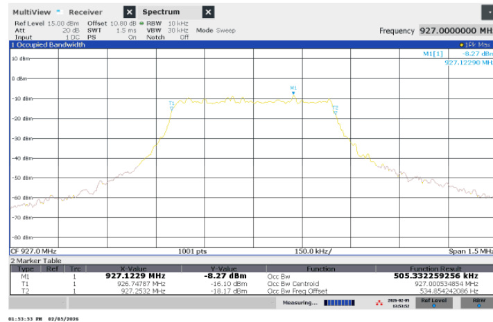
Figure 10 – 99% Bandwidth – Channel 16
