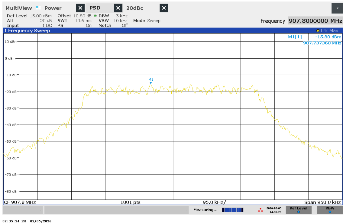
Figure 21 – PSD – Channel 4
