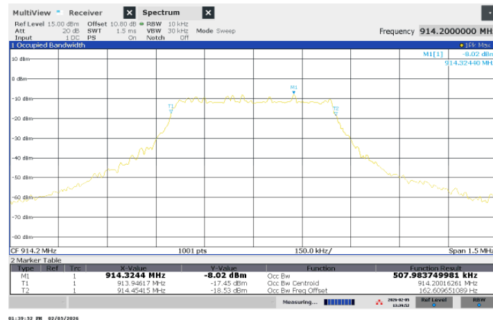
Figure 8 – 99% Bandwidth – Channel 8
