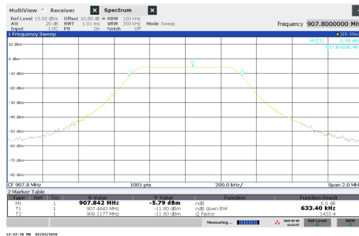
Figure 2 – 6dB Bandwidth – Channel 4
