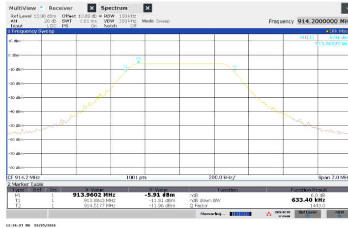
Figure 3 – 6dB Bandwidth – Channel 8
