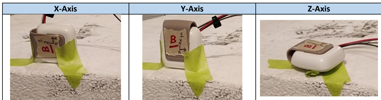
Figure 2 – DUT Orientations (Worst Case: Y-Axis)
